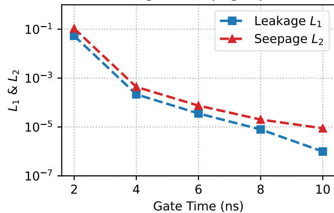
Leakage & Seepage ( \beta=1 )
