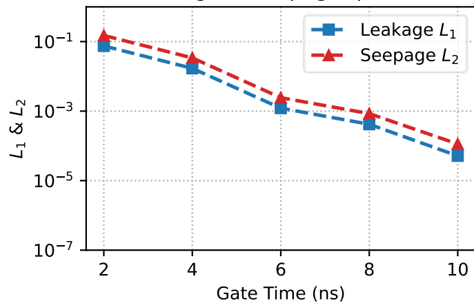
Leakage & Seepage ( \beta=0.5 )
