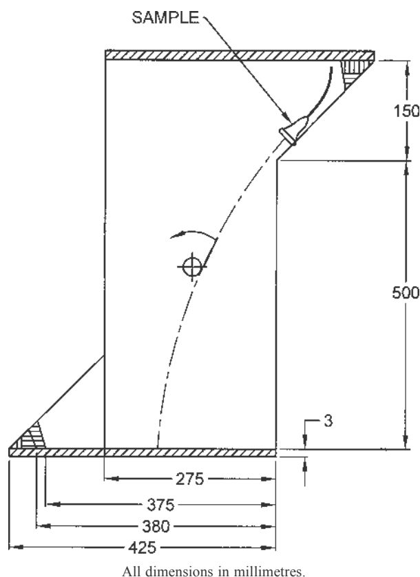
FIG. 26 TUMBLING BARREL
