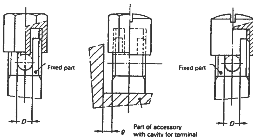
FIG. 5 MANTLE TERMINALS
