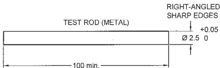
FIG. 35 GAUGE FOR VERIFICATION OF GROOVES, HOLES AND REVERSE TAPERS
