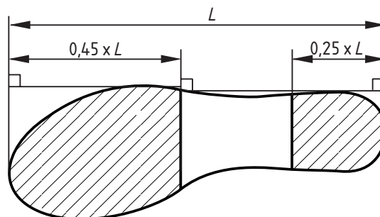
Figure 5 — Cleated area
