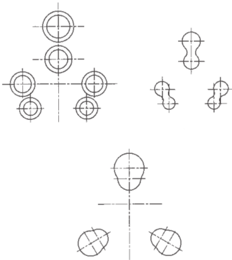
FIG. 1C COMBINED SOCKET-OUTLETS'
