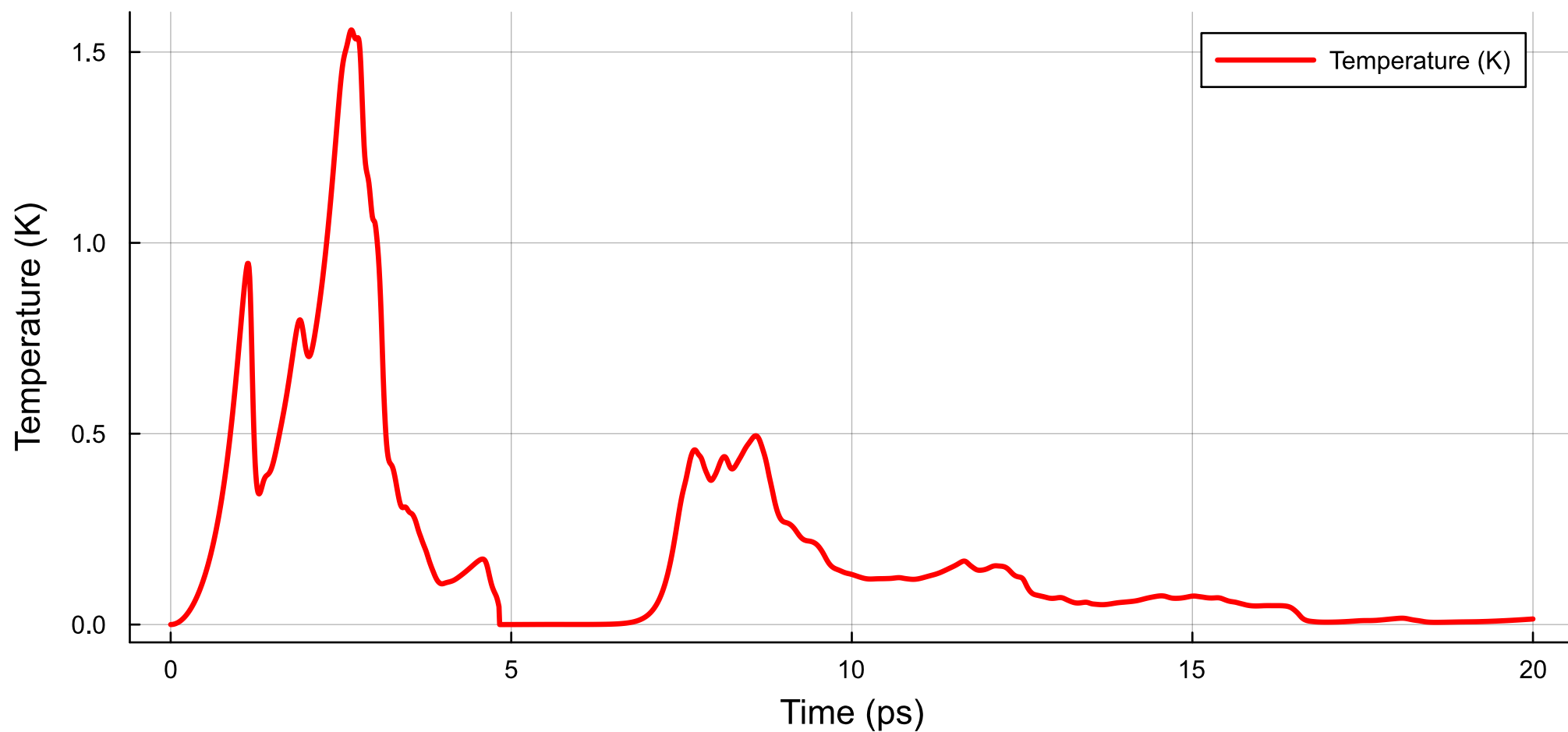
MD Simulation: Thermodynamic Quantities
