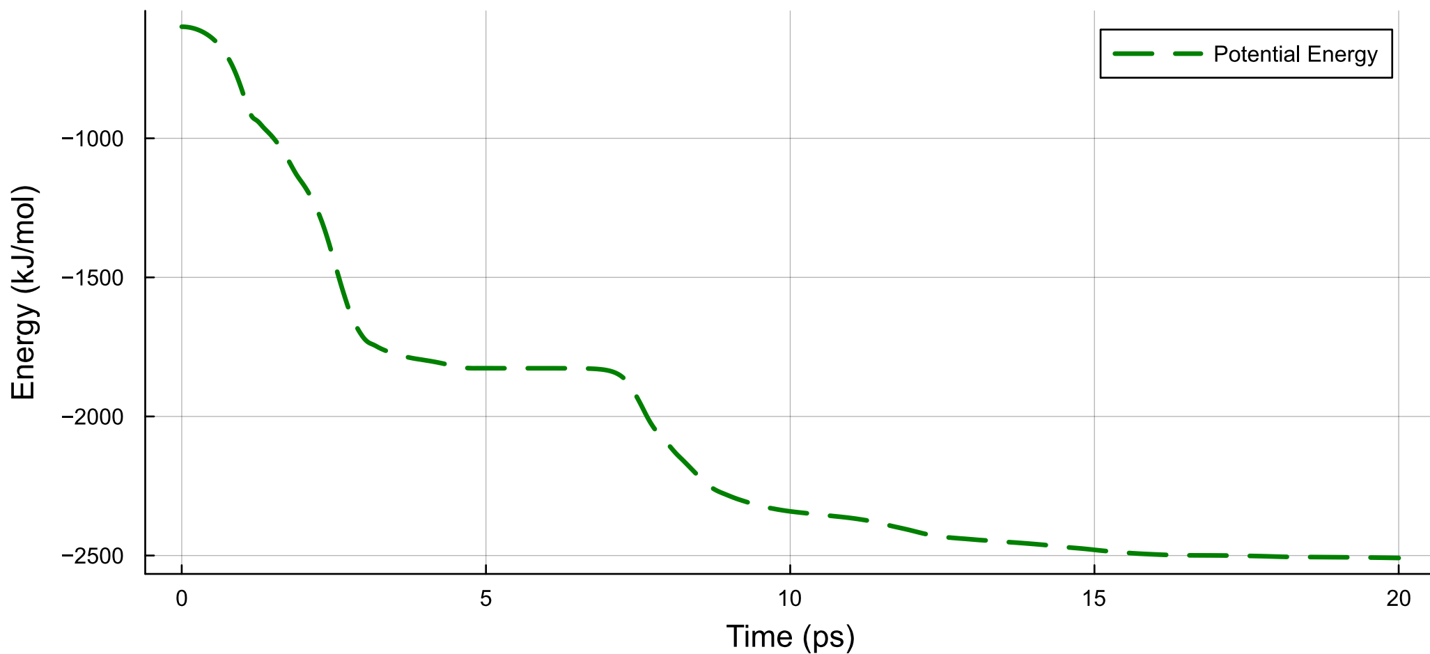
MD Simulation: Thermodynamic Quantities
