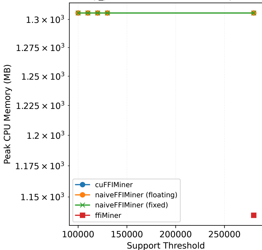
Fuzzy_pumb — Peak CPU Memory (MB)
