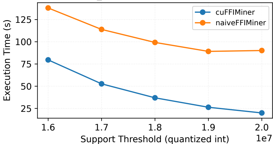
Fuzzy_pumsb — Execution Time (s)
