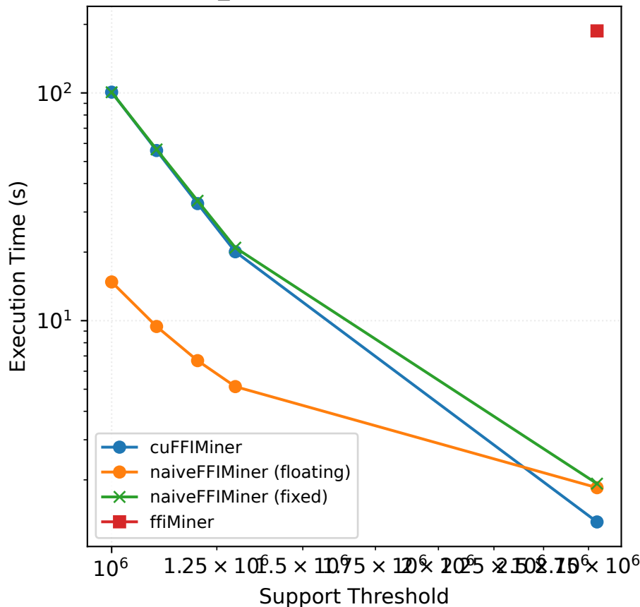
Fuzzy_pumsb — Execution Time (s)
