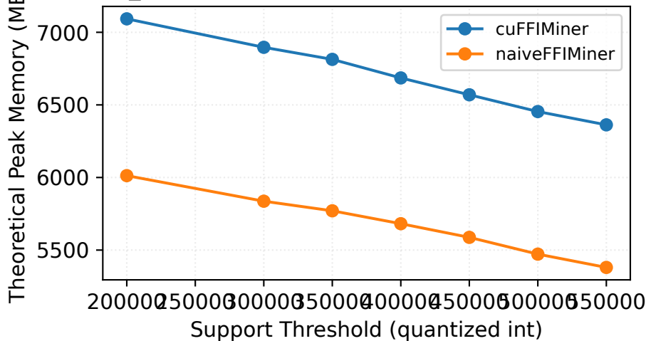
Fuzzy_T10I4D100K — Theoretical Peak Memory (MB)
