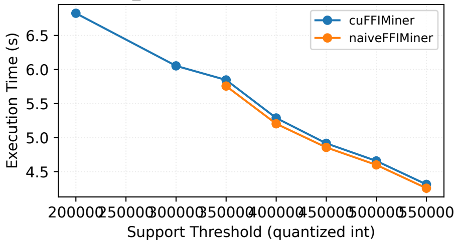
Fuzzy_T10I4D100K — Execution Time (s)
