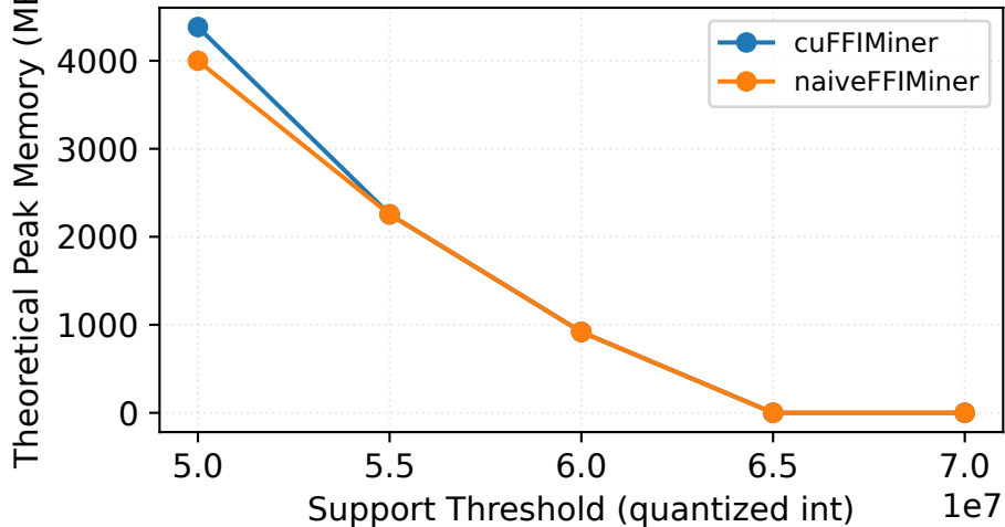
Fuzzy_connect — Theoretical Peak Memory (MB)
