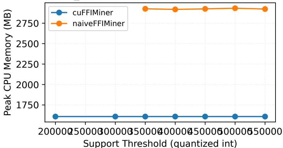
Fuzzy_T10I4D100K — Peak CPU Memory (MB)
