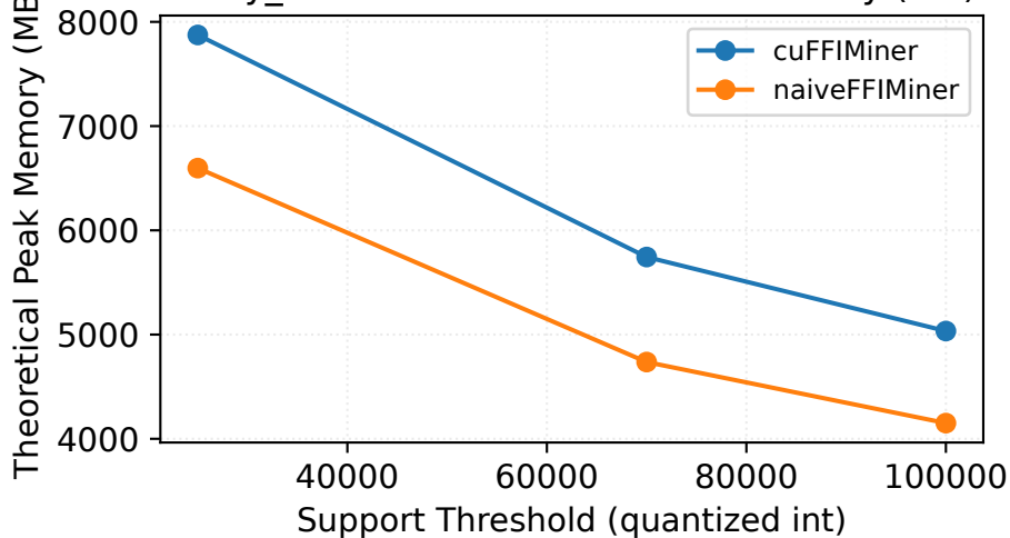
Fuzzy_retail — Theoretical Peak Memory (MB)
