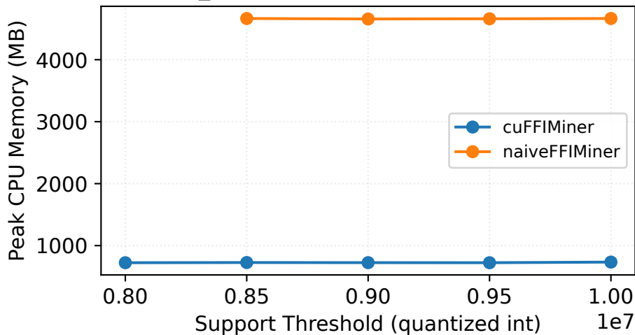
Fuzzy_connect — Peak CPU Memory (MB)
