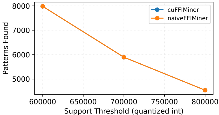
Fuzzy_kosarak - Patterns Found
