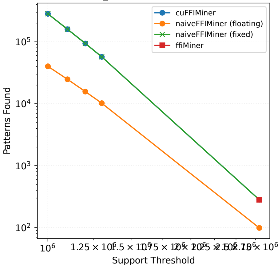
Fuzzy_pumb — Patterns Found
