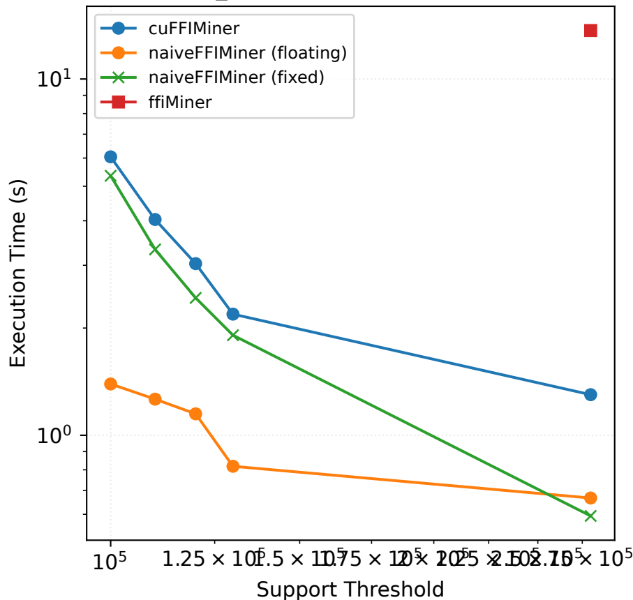
Fuzzy_pumb — Execution Time (s)
