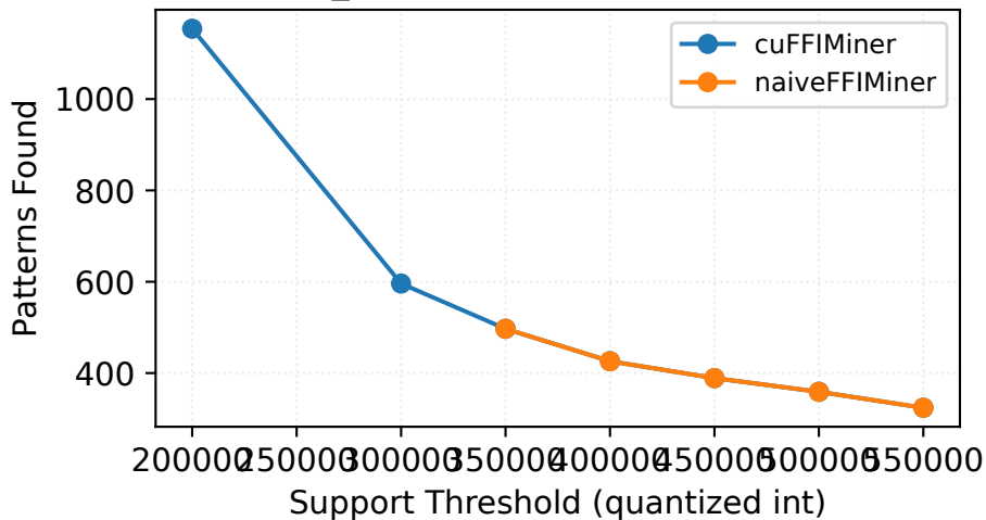
Fuzzy_T10I4D100K — Patterns Found
