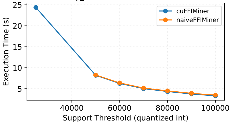
Fuzzy_retail — Execution Time (s)
