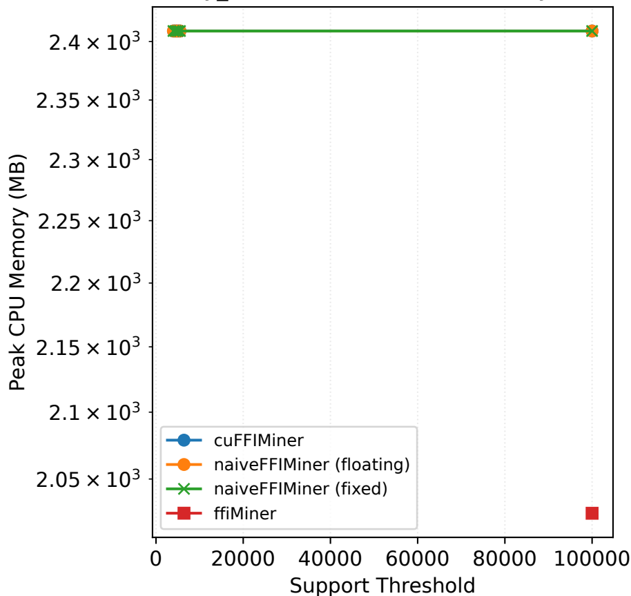
Fuzzy_kosarak — Peak CPU Memory (MB)
