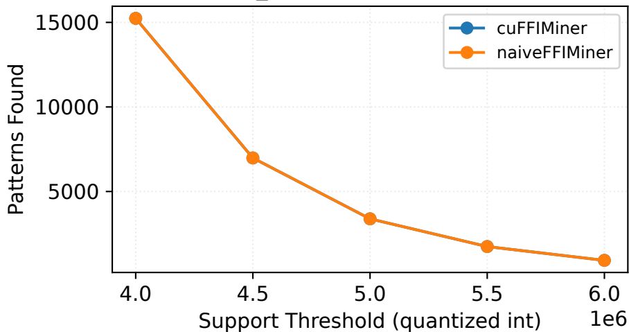
Fuzzy_pumsb — Patterns Found
