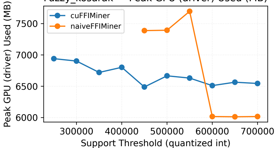
Fuzzy_kosarak — Peak GPU (driver) Used (MB)
