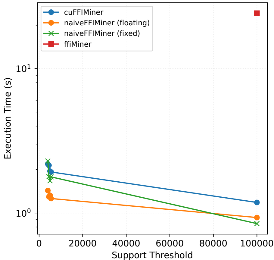
Fuzzy_kosarak — Execution Time (s)
