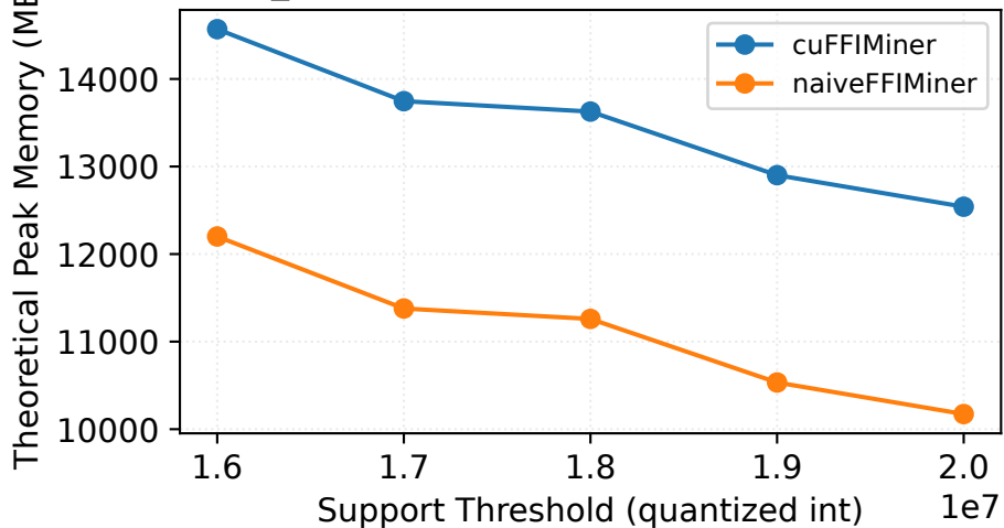
Fuzzy_pumsb — Theoretical Peak Memory (MB)
