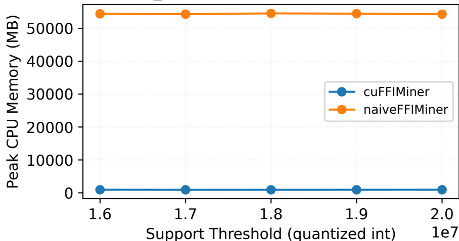
Fuzzy_pumsb — Peak CPU Memory (MB)
