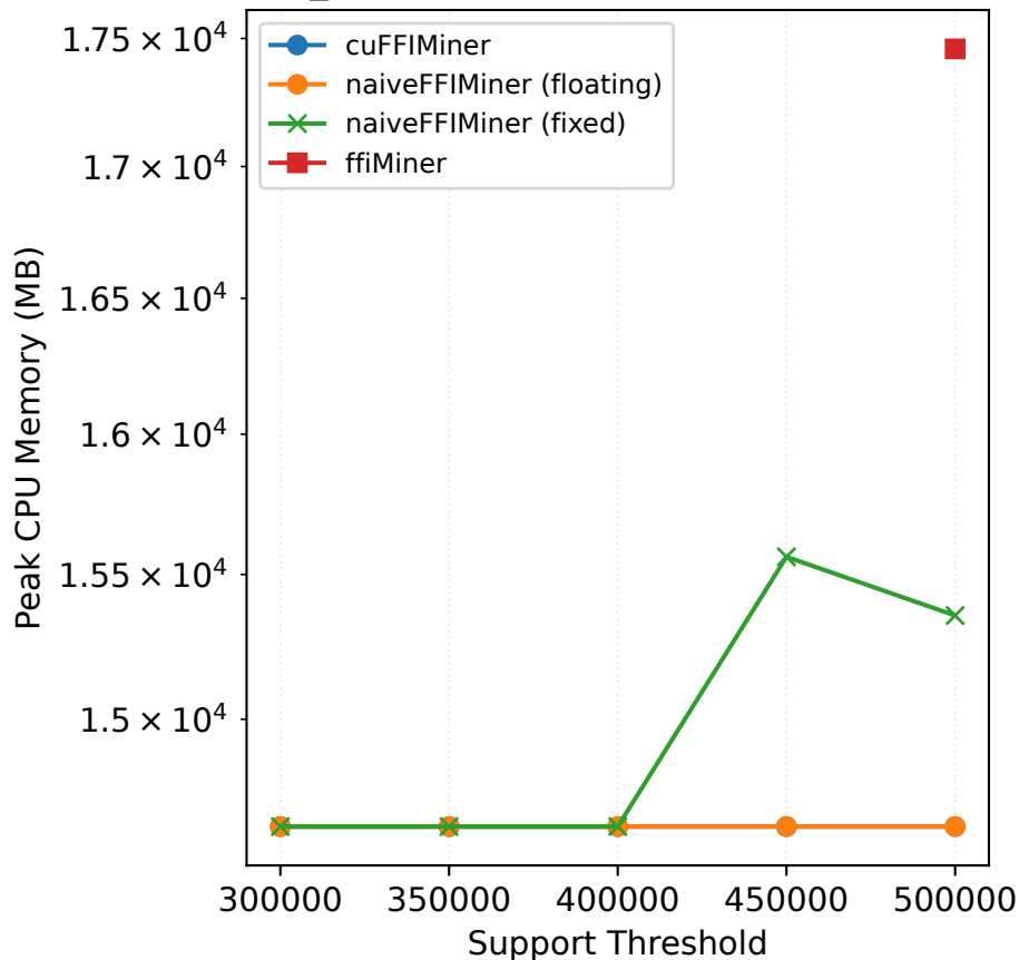
Fuzzy_T10I4D100K — Peak CPU Memory (MB)
