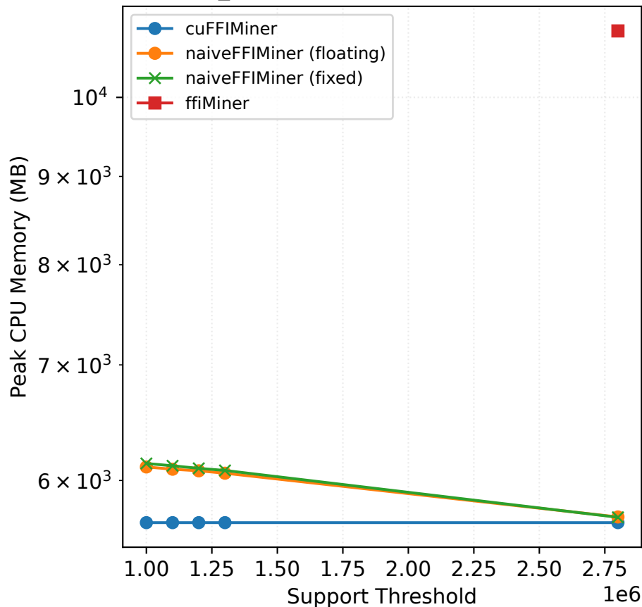
Fuzzy_pumsb — Peak CPU Memory (MB)
