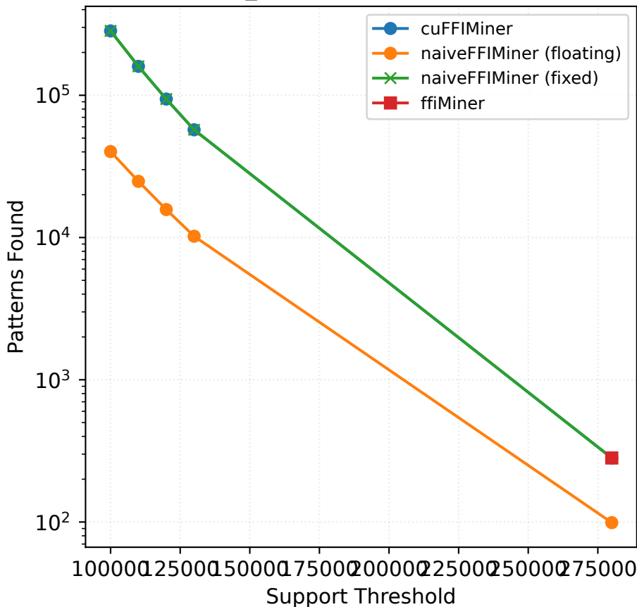
Fuzzy_pumsb — Patterns Found
