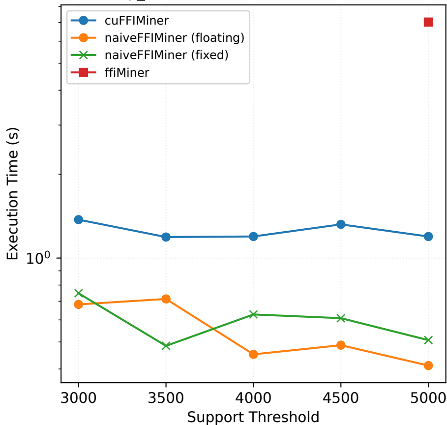
Fuzzy_T10I4D100K — Execution Time (s)
