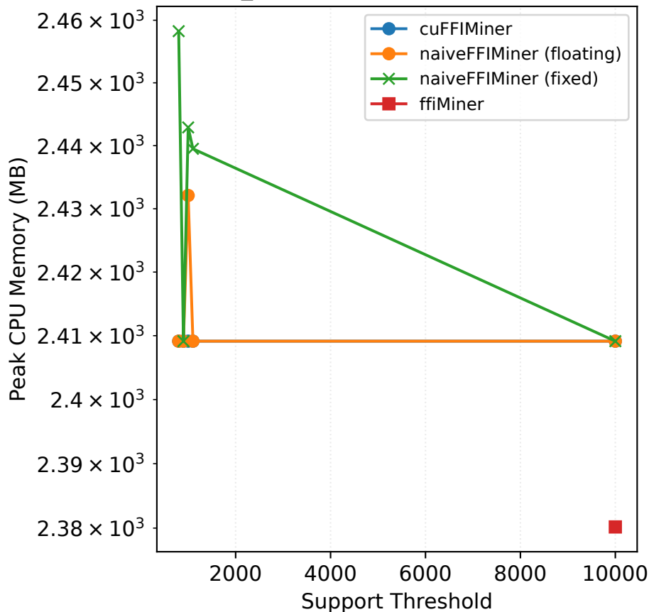
Fuzzy_retail — Peak CPU Memory (MB)
