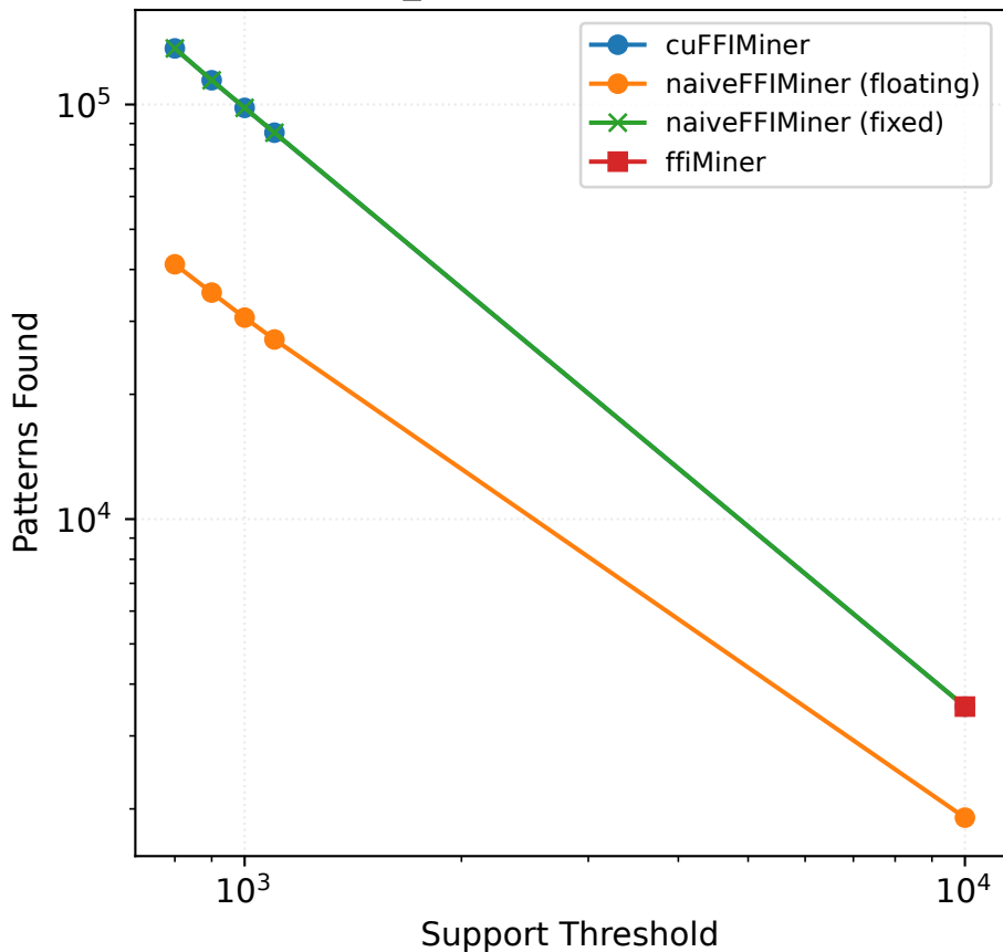
Fuzzy_retail — Patterns Found
