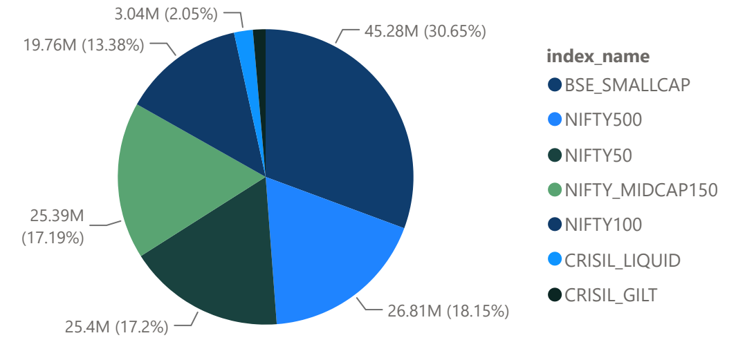
Benchmark comparison
