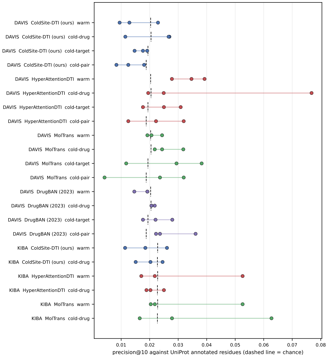
One cell, three training seeds: a verdict that moves across chance
