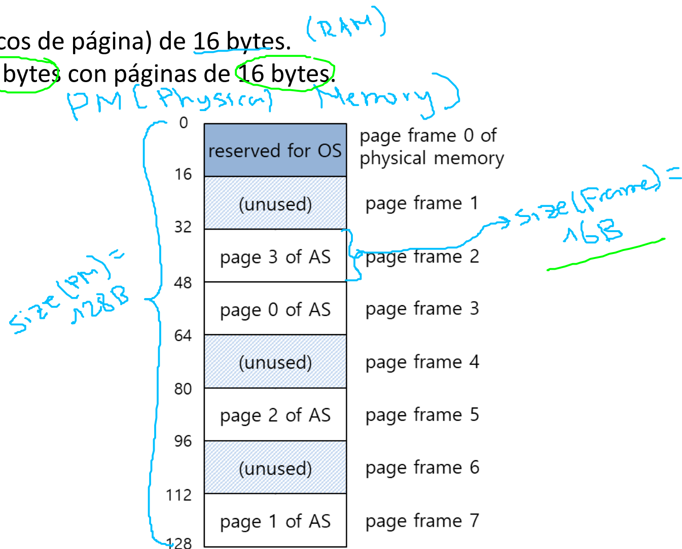
64-Byte Address Space Placed In Physical Memory
