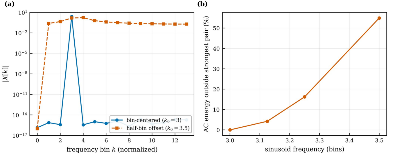
Figure S7. Spectral leakage for bin-centered and off-bin sinusoids.
