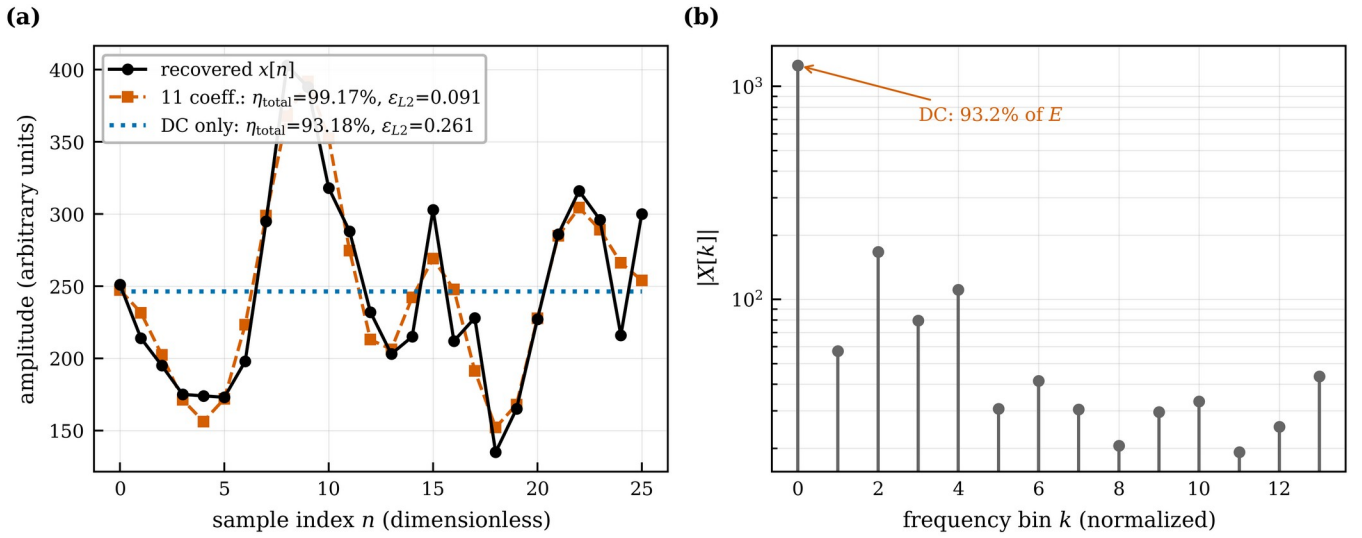
Figure S1. Recovered baseline sequence, its 11-coefficient and DC-only reconstructions, and the magnitude spectrum.
