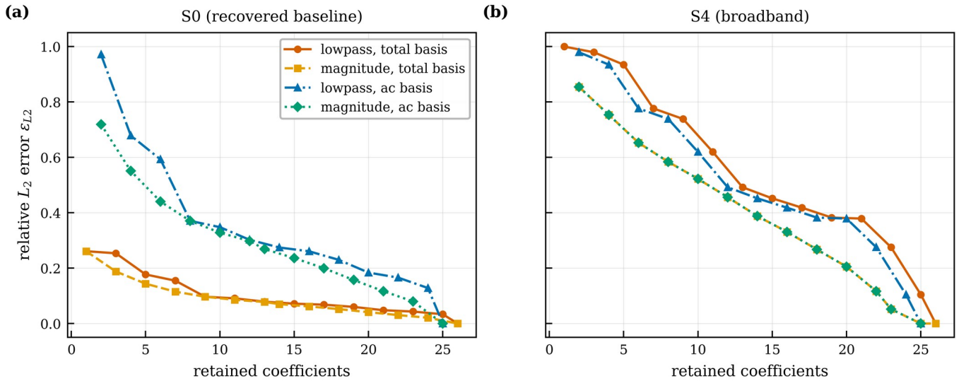
Figure S5. Coefficient count against reconstruction error for all strategy and basis combinations.
