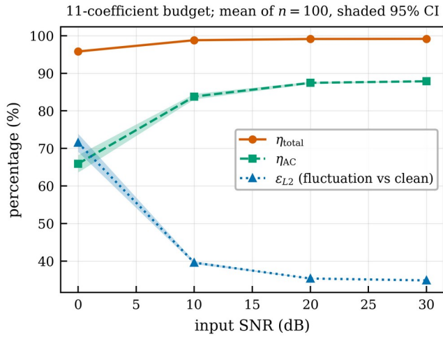
Figure S9. Retention and fidelity against input
