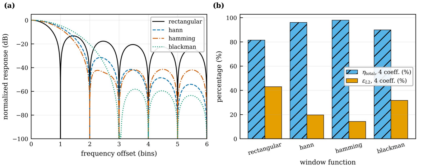
Figure S8. Window frequency responses and their effect at a fixed coefficient budget.
