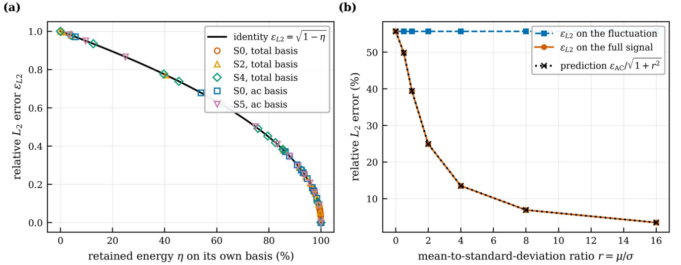
Figure S3. The redundancy result: all retention curves lie exactly on the identity, and the two error
