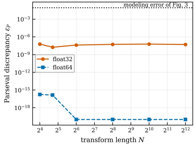
Figure S10. Parseval discrepancy against transform length and floating-point precision.
