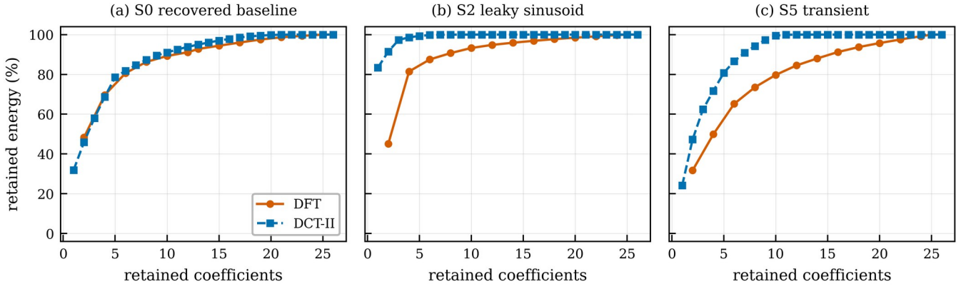
Figure S6. DFT against orthonormal DCT-II compaction, mean-removed.
