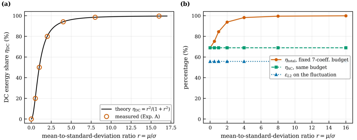
Figure S2. Experiment A: measured DC energy share against the analytical prediction, and the divergence of retention from fidelity as the offset grows.
