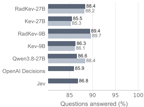
a Coverage at 5% error
