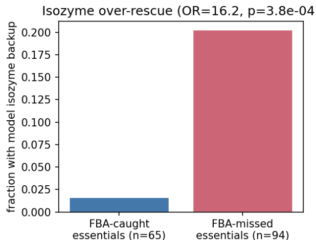
Figure 3: Isozyme over-rescue: FBA-missed essentials carry model isozyme backups at 13\times the rate of FBA-caught essentials.
