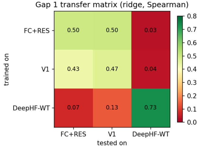
Figure 2: Gap 1 transfer matrix (ridge, seed 0): within-family transfer is moderate (0.43--0.50) but every cross-family entry collapses to \leq 0.13 , against within-screen 0.73. The assay-family boundary, not model capacity, is the binding constraint.
