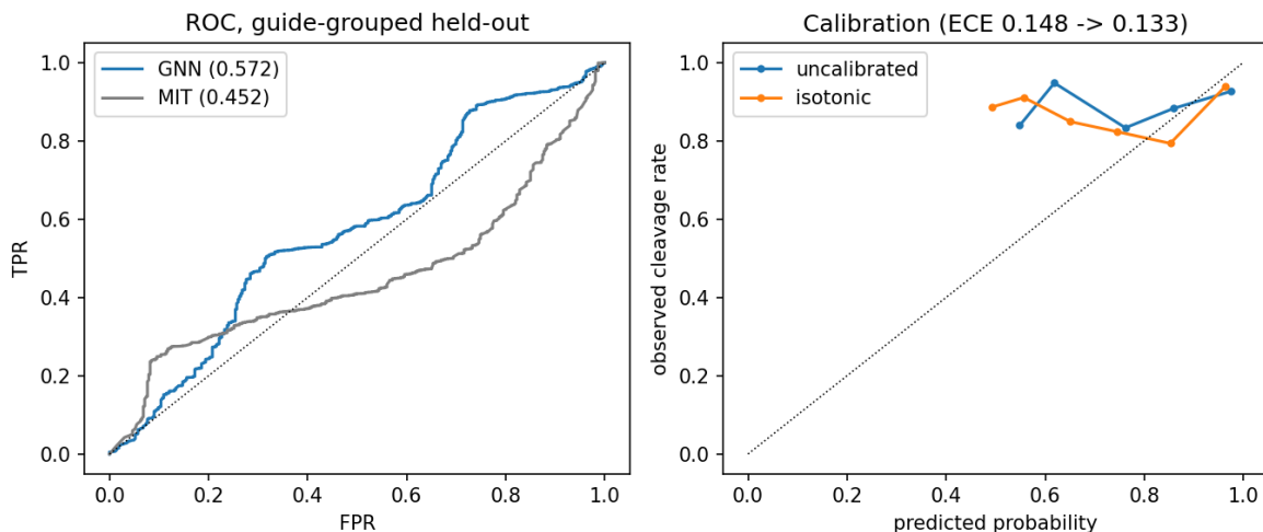
Figure 3: Gap 2, guide-grouped held-out crisprSQL, seed-0 split. Left: ROC for the GNN and the MIT score. Right: calibration before/after isotonic regression; the corpus’s 91% test prevalence compresses the curve into the high range, where isotonic still reduces ECE.
