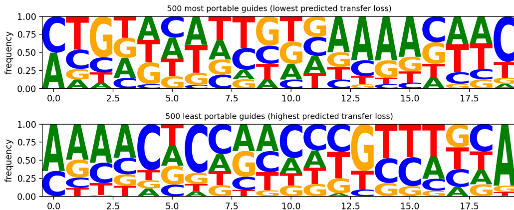
Figure 8: Sequence logos of the 500 most vs least portable DeepHF WT guides under the reconstructed PORTA pipeline (held-out score–residual \rho = 0.825 ). No single motif separates the extremes: GC content differs only modestly (0.436 vs 0.496) and composition differences are positional and weak – direct visual evidence for the distributed signature behind the residual (Section 12).
