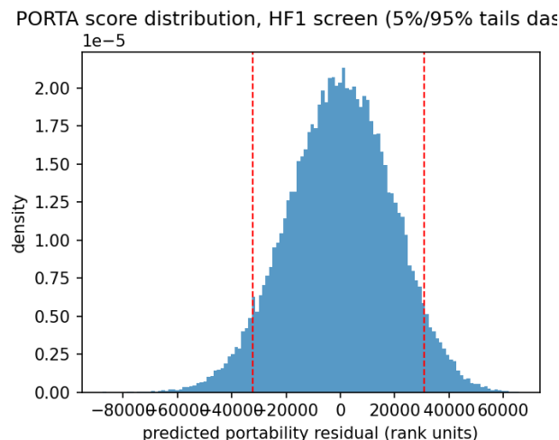
Figure 16: Distribution of the predicted portability residual on the HF1 screen; dashed lines mark the 5%/95% tails (guides the source model systematically over- or under-ranks).
