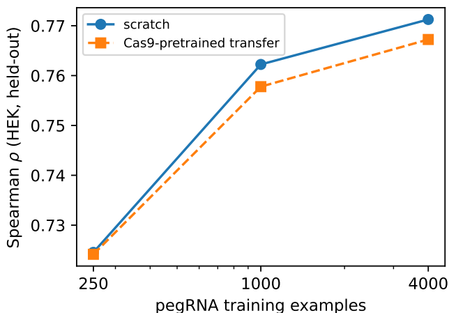
Figure 10: Scarce-regime scaling: Cas9-motif transfer never beats scratch.
