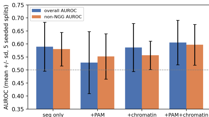
Figure 11: Gaps 4–5 channel ablation, five fully-seeded splits (mean \pm sd). Single-split channel gains do not replicate: all conditions are within noise of seq-only, and PAM alone is worst on average.
