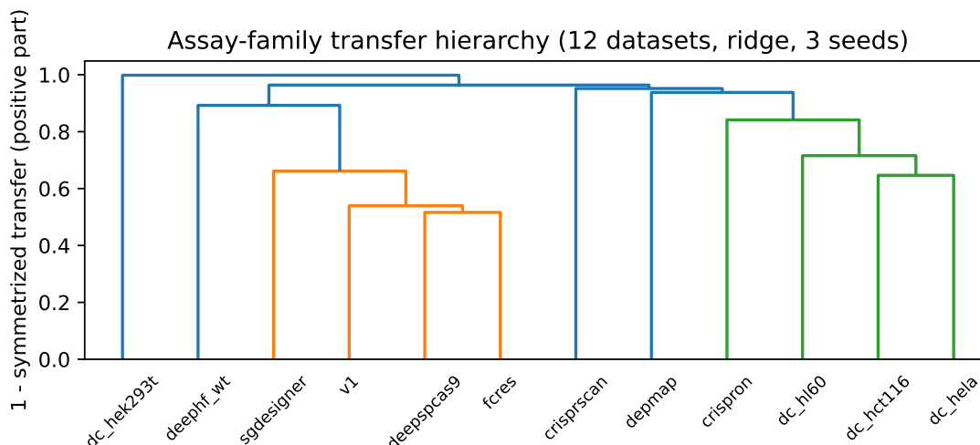
Figure 6: Average-linkage hierarchy (scipy) on the symmetrized positive-part transfer similarity across the 12 gap-1 datasets. The Wang/Xu-side family (HCT116, HeLa, HL60, CRISPRon) clusters tightly; DepMap and CRISPRscan attach weakly to it; the HEK family (fcres/v1/DeepSpCas9/sgDesigner/DeepHF) forms the other subtree, with the anomalous Deep-CRISPR HEK293T set joining last. Independent confirmation of the Louvain partition.
