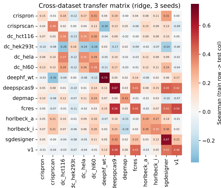
Figure 5: The full 14 \times 14 cross-dataset transfer matrix (ridge, mean of 3 seeds; diagonal = within-dataset). The HEK-nuclease block (bottom right) and the Wang/Xu block (upper middle) are visible as coherent red squares; the DeepCRISPR-HEK293T column is uniformly blue (the inversion anomaly); the Horlbeck CRISPRi/a pair transfers to each other and to sgDesigner/CRISPRscan but negatively to DepMap.
