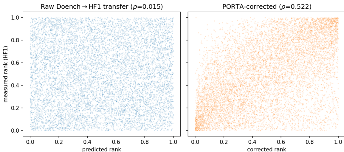
Figure 15: PORTA correction on SpCas9-HF1. Left: raw Doench→HF1 transfer ranking vs measured ranks ( \rho = 0.015 , no visible structure). Right: after subtracting the WT-trained portability model ( \rho = 0.522 ).
