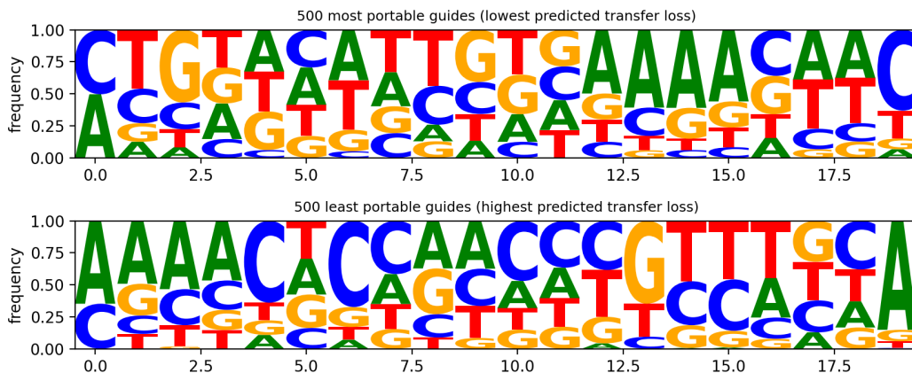
Figure 9: Sequence logos of the 500 most vs least portable DeepHF WT guides under the re-constructed PORTA pipeline (held-out score–residual \rho = 0.825 ). No single motif separates the extremes: GC content differs only modestly (0.436 vs 0.496) and composition differences are positional and weak – direct visual evidence for the distributed signature behind the residual (Section 12).
