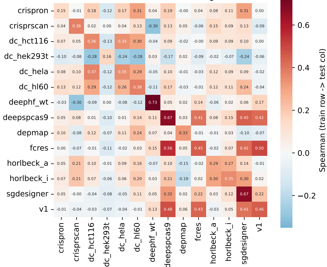
Cross-dataset transfer matrix (ridge, 3 seeds)
