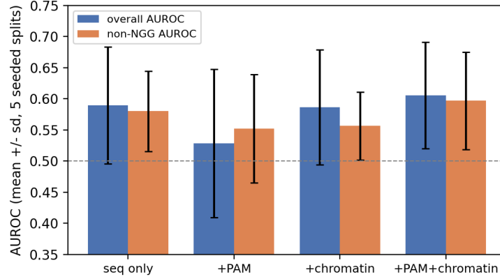
Figure 6: Gaps 4–5 channel ablation, five fully-seeded splits (mean \pm sd). Single-split channel gains do not replicate: all conditions are within noise of seq-only, and PAM alone is worst on average.
