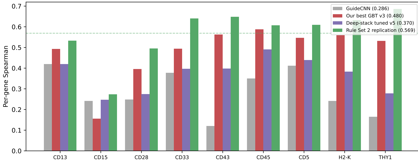
Clean protocol (train RES human, test V1 mouse): same-split Rule Set 2 replication remains unbeaten
