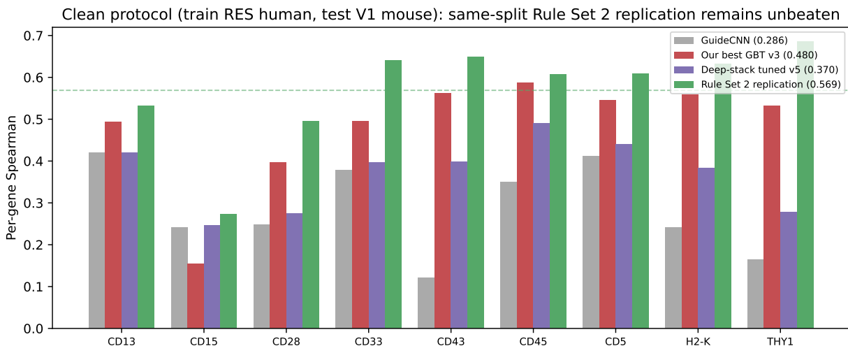
Figure 5: Per-gene Spearman on V1 under the clean Azimuth cross-dataset protocol (train RES only). All our current models sit below the same-split Rule Set 2 replication (0.569); the earlier contaminated run that appeared to exceed the old bar is retracted.
