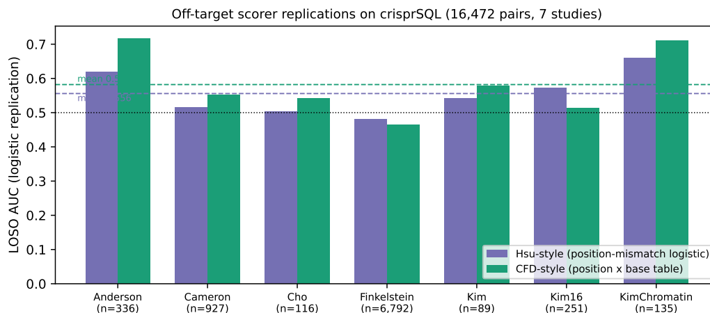
Figure 10: Per-study LOSO AUC for the Hsu-style and CFD-style replications on crisprSQL (results/offtarget_scorers.json). CFD-style wins 5 of 7 studies, matching the published ordering - the harness reproduces known reference behavior before we trust it with new claims.
