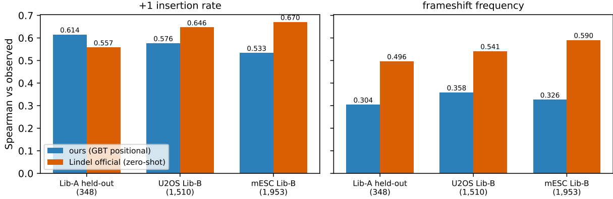
Figure 4: Tool 7 transfer matrix (Spearman vs observed, real inDelphi data): our GBT wins the in-distribution +1-insertion comparison on held-out Lib-A but loses every transfer comparison to the official Lindel model run zero-shot.
