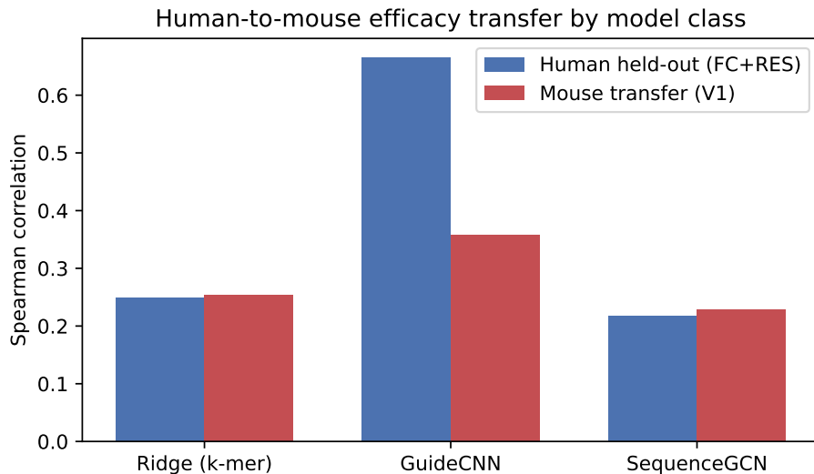
Figure 7: Human-held-out versus mouse-transfer Spearman by model class. Only the CNN leads on both axes but pays a real transfer penalty (0.665 RES held-out to 0.358 mouse V1); the simple baselines are flat.
