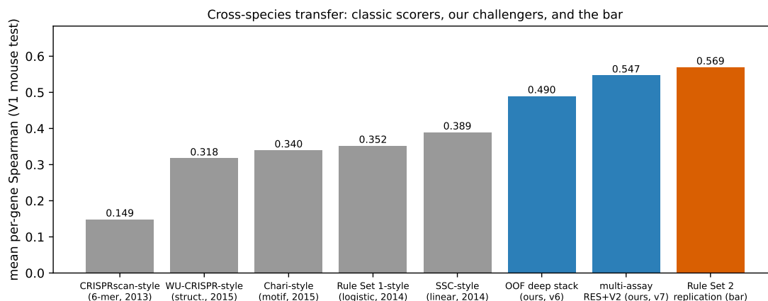
Figure 9: Classic efficacy scorers replicated on the clean RES→V1 split (results/classic_scorers.json) against our challengers (v6, v7) and the same-split Rule Set 2 replication bar. The published ordering (CRISPRscan < Rule Set 1 < SSC < Rule Set 2) reproduces, and no challenger reaches the bar.
