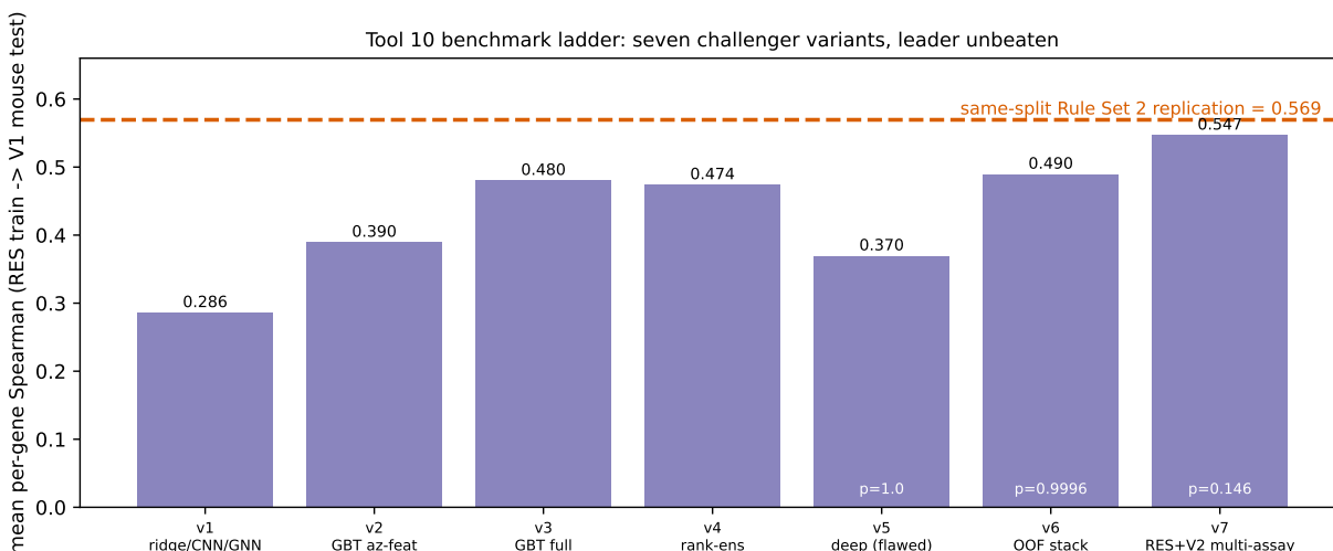
Figure 8: The Tool 10 benchmark ladder on the clean RES-human \rightarrow V1-mouse split (mean per-gene Spearman), built at compile time from the committed results/beat_azimuth_v*.json files by scripts/make_figures7.py . The orange dashed line is the same-split Rule Set 2 replication (0.569), the honest bar. Seven challenger variants - ridge/CNN/GNN featurizations (v1, best of the three shown), GBT on Azimuth features (v2, v3), a GBT rank ensemble (v4), a deep stack with a leaked normalization (v5, flawed and retracted), a leak-free out-of-fold deep stack (v6), and multi-assay RES+V2 training (v7) - all lose; paired bootstrap p -values over genes are printed inside the bars where computed. The ladder is the honest record of a benchmark we tried seven ways to break and did not.
