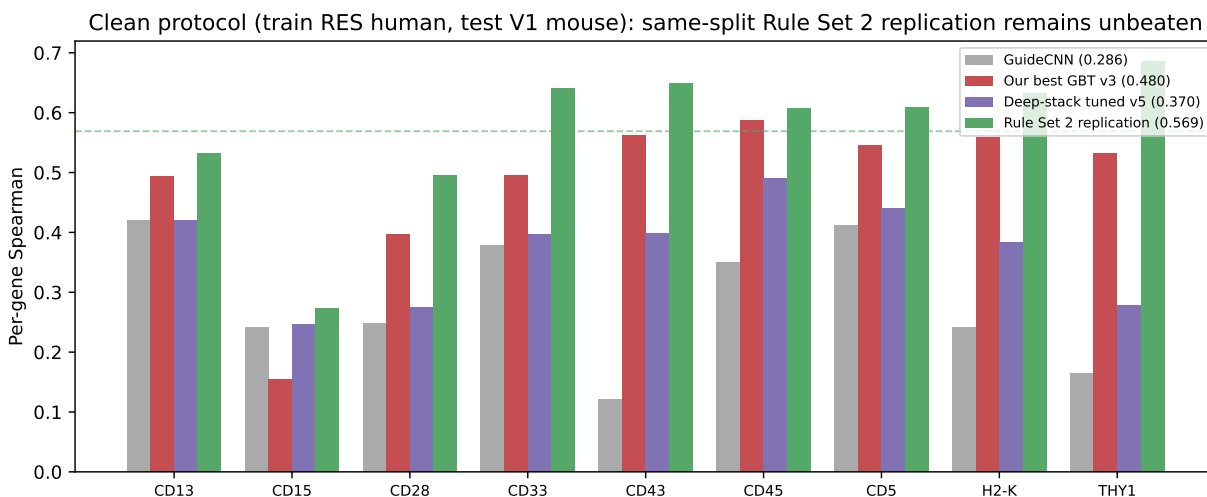
Figure 11: Per-gene Spearman on V1 under the clean Azimuth cross-dataset protocol (train RES only). All our current models sit below the same-split Rule Set 2 replication (0.569); the earlier contaminated run that appeared to exceed the old bar is retracted.
