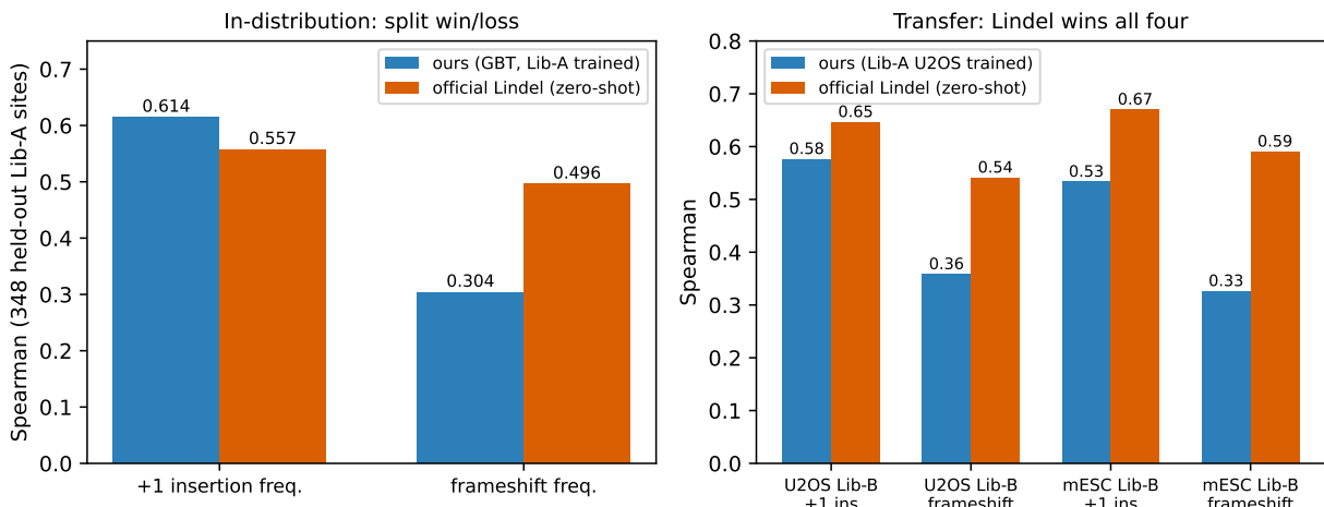
Figure 3: Head-to-head against the official Lindel model, all numbers from results/lindel_headtohead.json and results/outcome_crosscell.json . Left: in-distribution, 348 held-out Lib-A sites - our GBT wins the +1-insertion rate (0.614 vs 0.557) and loses frameshift frequency (0.304 vs 0.496). Right: the same comparison transferred to Lib-B loci in U2OS and in mESC - Lindel wins all four transfer evaluations, so the in-distribution win does not generalize across loci, cell line, or species.
