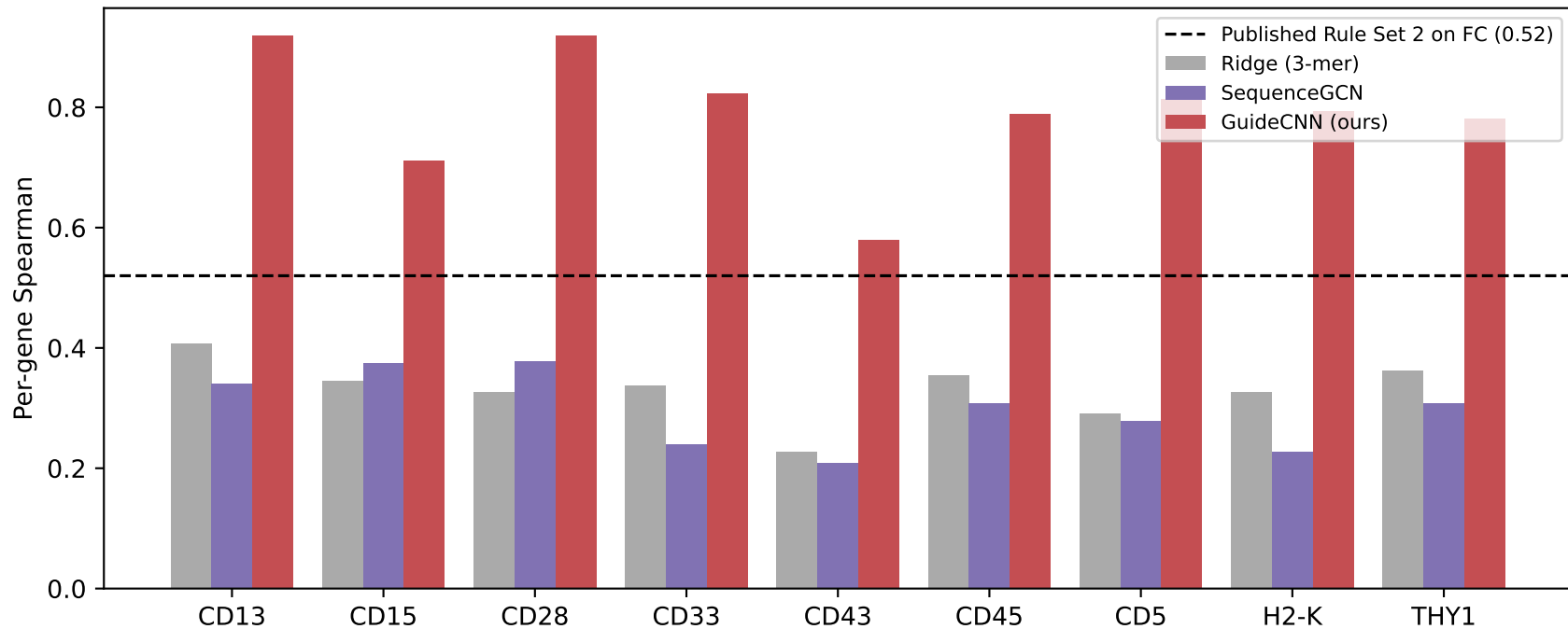
Cross-dataset protocol (train RES, test V1/FC): GuideCNN vs published Rule Set 2
