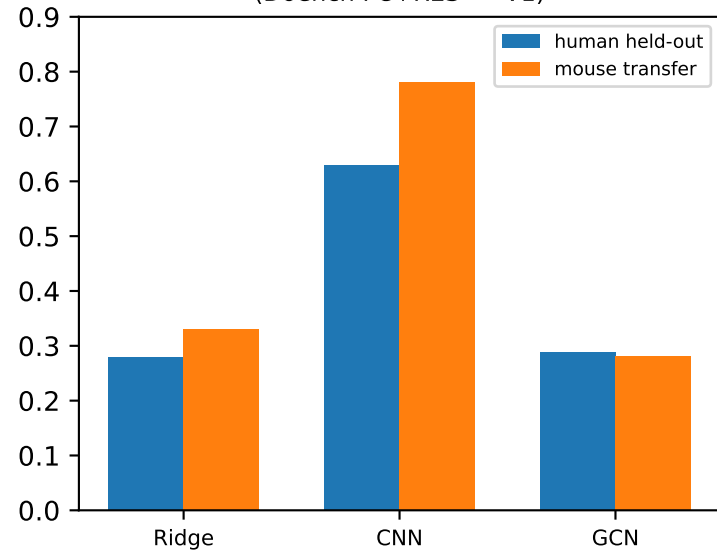
Tool 10: human->mouse transfer (Doench FC+RES -> V1)
