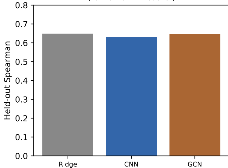
Tool 6: duplex-MFE surrogate (vs ViennaRNA teacher)
