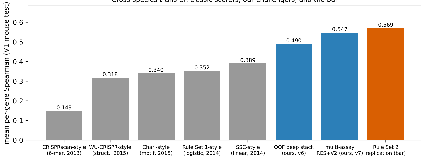
Cross-species transfer: classic scorers, our challengers, and the bar
