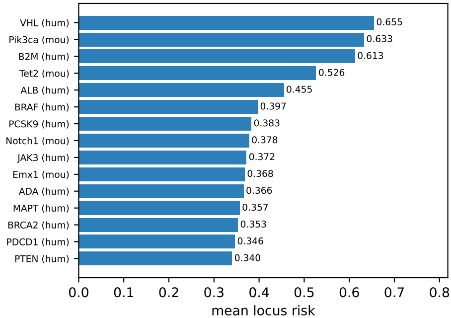
Top 15 loci by mean risk
