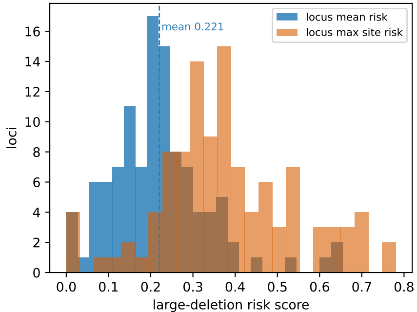
Tool 8 panel: 109 loci, 478 cut sites
