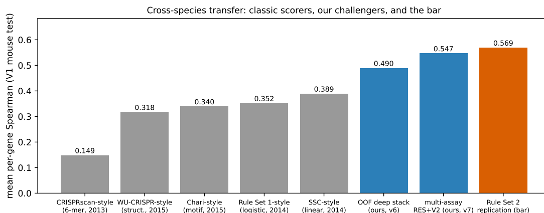
Figure 9: Classic efficacy scorers replicated on the clean RES→V1 split ( results/classic_scorers.json ) against our challengers (v6, v7) and the same-split Rule Set 2 replication bar. The published ordering (CRISPRscan < Rule Set 1 < SSC < Rule Set 2) reproduces, and no challenger reaches the bar.
