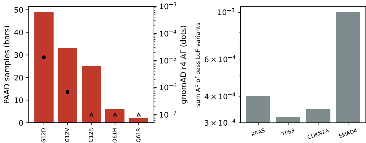
Figure 7: Left: the five KRAS alleles recurrent in PAAD (bars) against their gnomAD r4 allele frequencies (dots, log scale; open triangles mark alleles absent from gnomAD r4, plotted at the 10^{-7} floor). Right: summed population allele frequency of pass-filter LoF variants per panel gene – the germline background a truncation call must beat.
