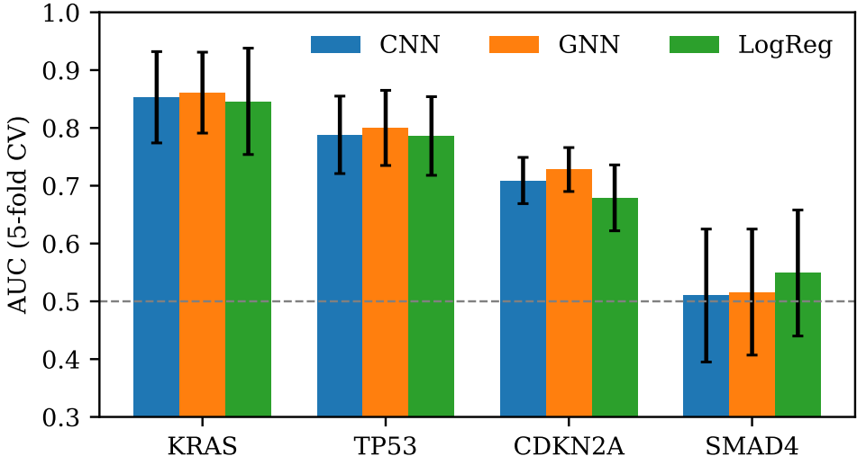
Figure 2: Mutation-prediction AUC (5-fold CV, mean \pm sd) for the four canonical PDAC drivers.
