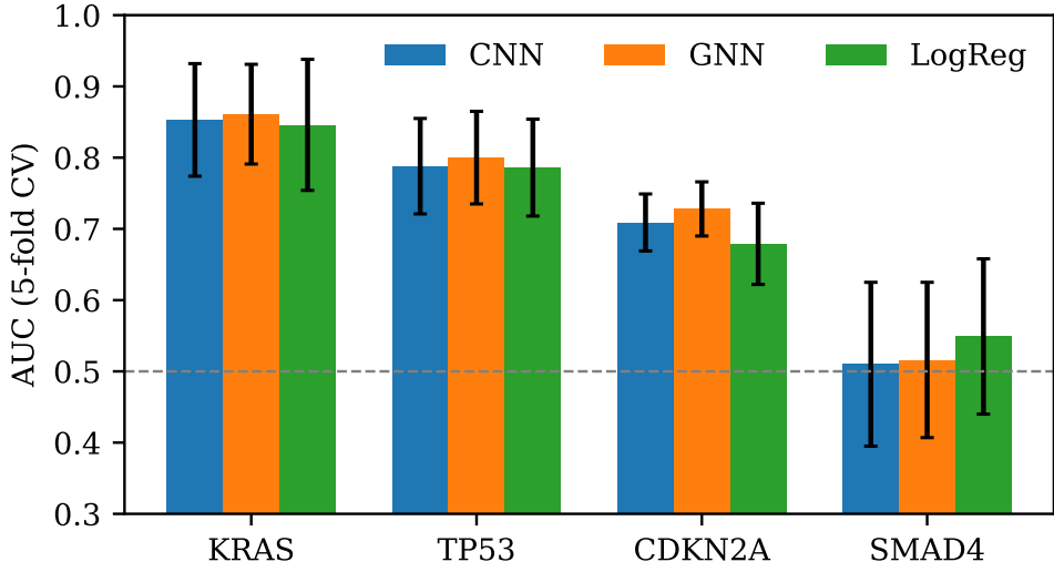
Figure 1: Mutation-prediction AUC (5-fold CV, mean \pm sd) for the four canonical PDAC drivers.
