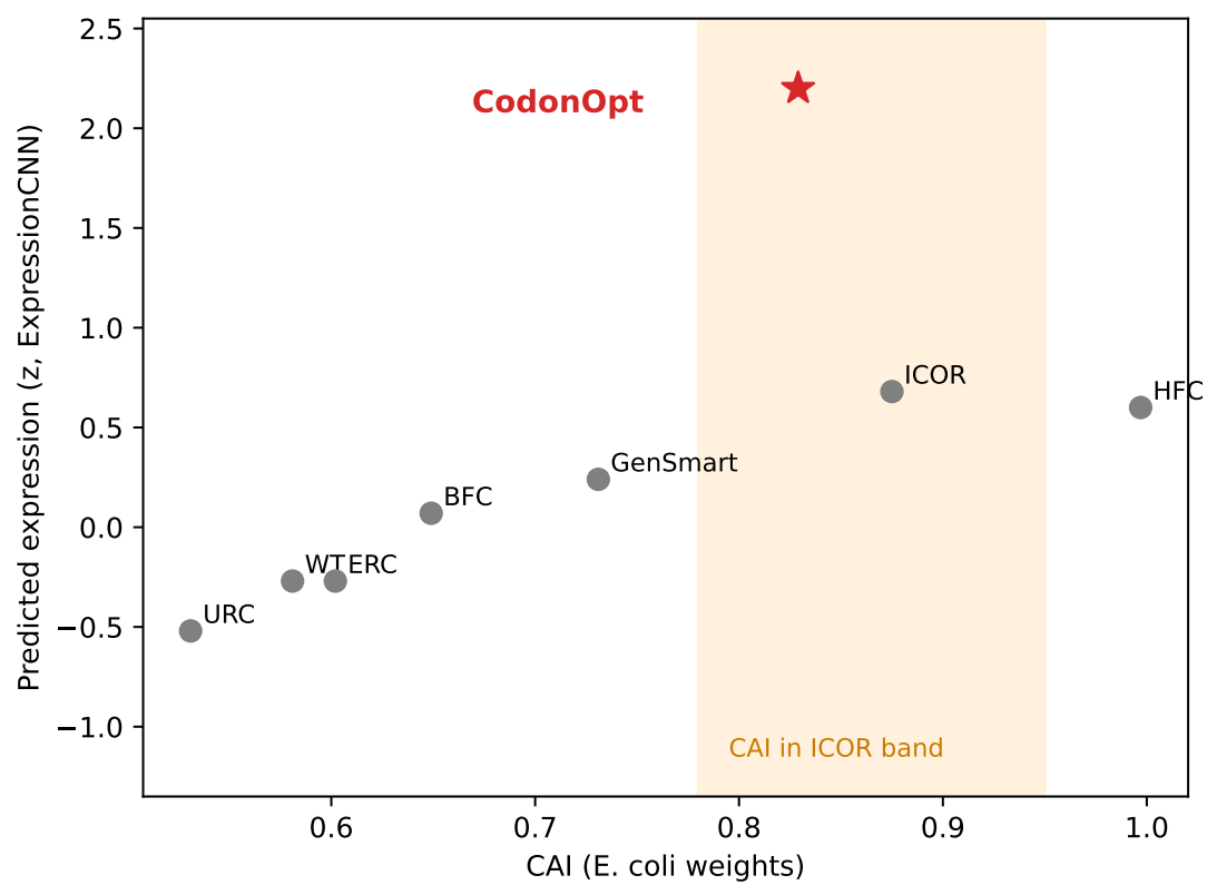
Figure 1: Central figure: CodonOpt vs ICOR, GenSmart and heuristic baselines on the published 40-gene benchmark. Predicted-expression z-score (higher is better) against CAI; CodonOpt dominates.
