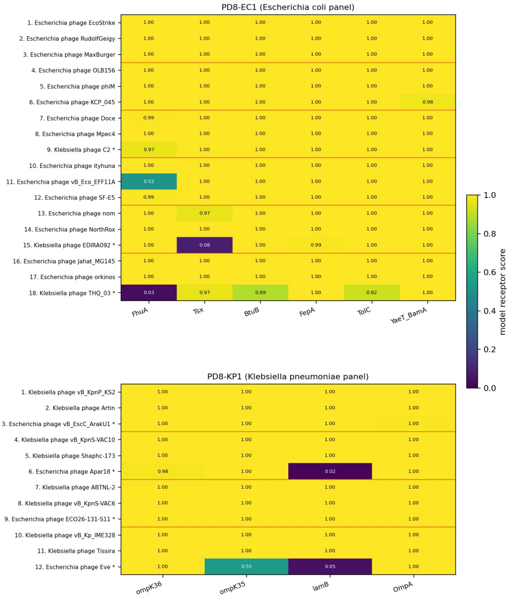
Figure 11. Cocktail member-by-targeted-receptor score heatmaps for PD8-EC1 (top, 18 members) and PD8-KP1 (bottom, 12). Rows are grouped by targeted receptor (red separators every k = 3 members); starred rows are discovery-candidate seats. The off-argmax saturation (many 1.00 cells outside the argmax class) is the calibration fact that makes argmax the only honest usage claim; within-class assignment is nevertheless sharp, with argmax scores 1.00 for 29 of 30 members (KP1.12 Eve: 0.998).
