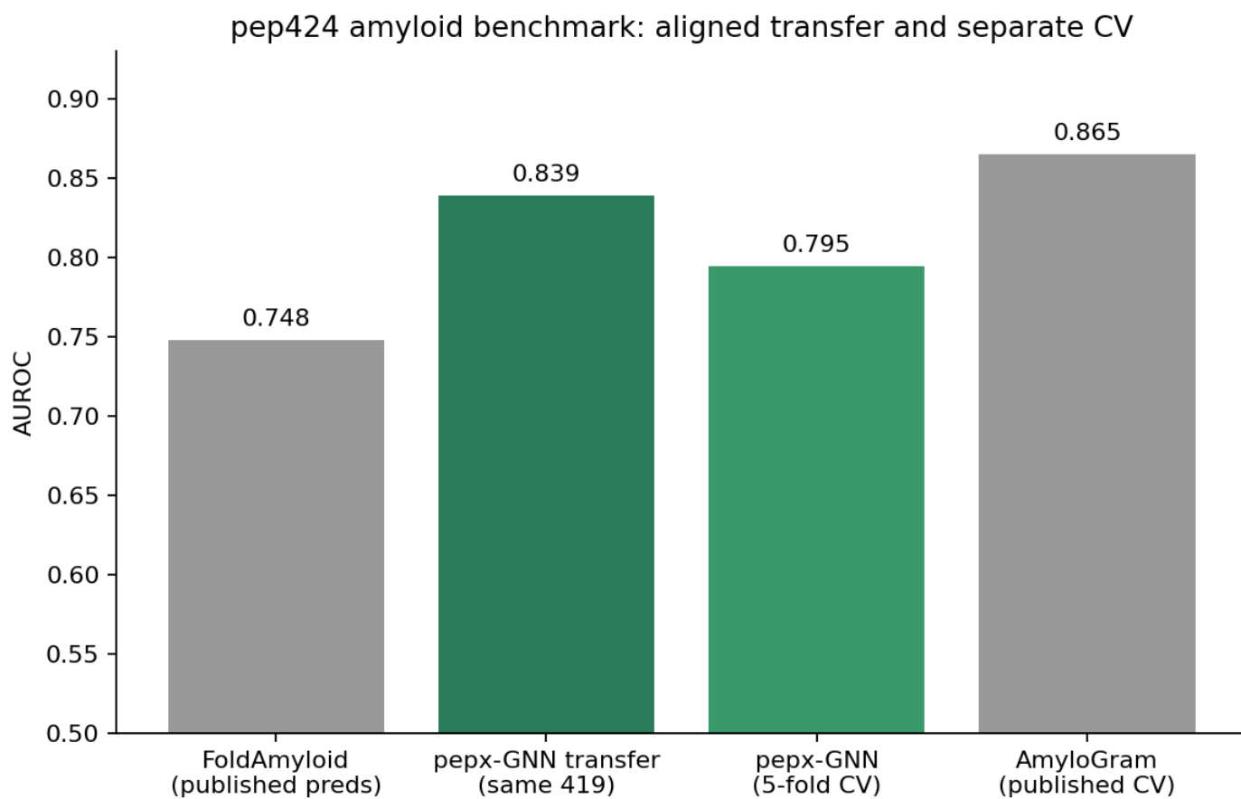
Figure 2: pep424 aligned head-to-head: transfer GNN 0.839 versus FoldAmyloid published predictions 0.748 on 419 identical sequences; separate CV results 0.795 and 0.865 are not the same-split comparison.
