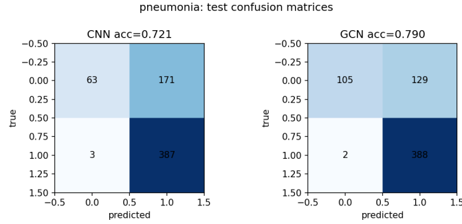
Figure 5: Pneumonia test-set confusion, RegionGCN (624 held-out official test images). Sensitivity is near-perfect; errors concentrate on the normal class.
