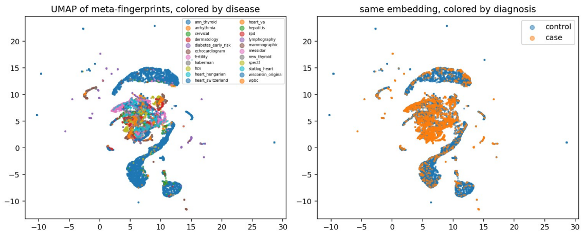
fingerprint umap
