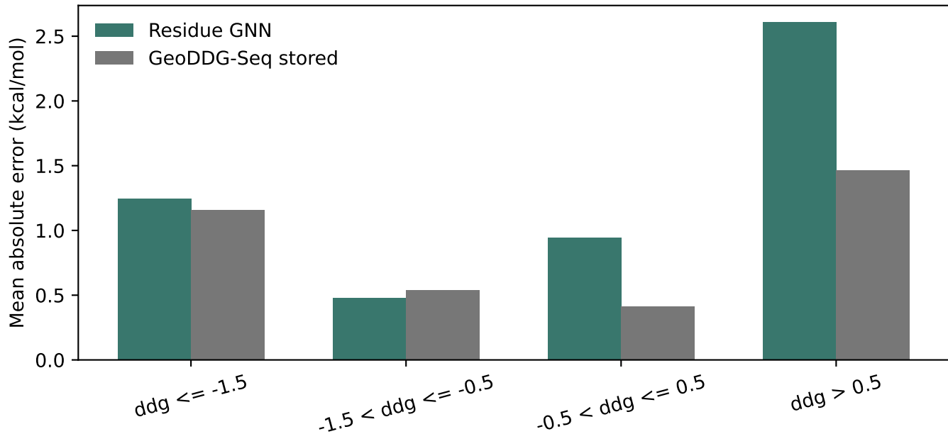
Error by observed DDG interval; exploratory
