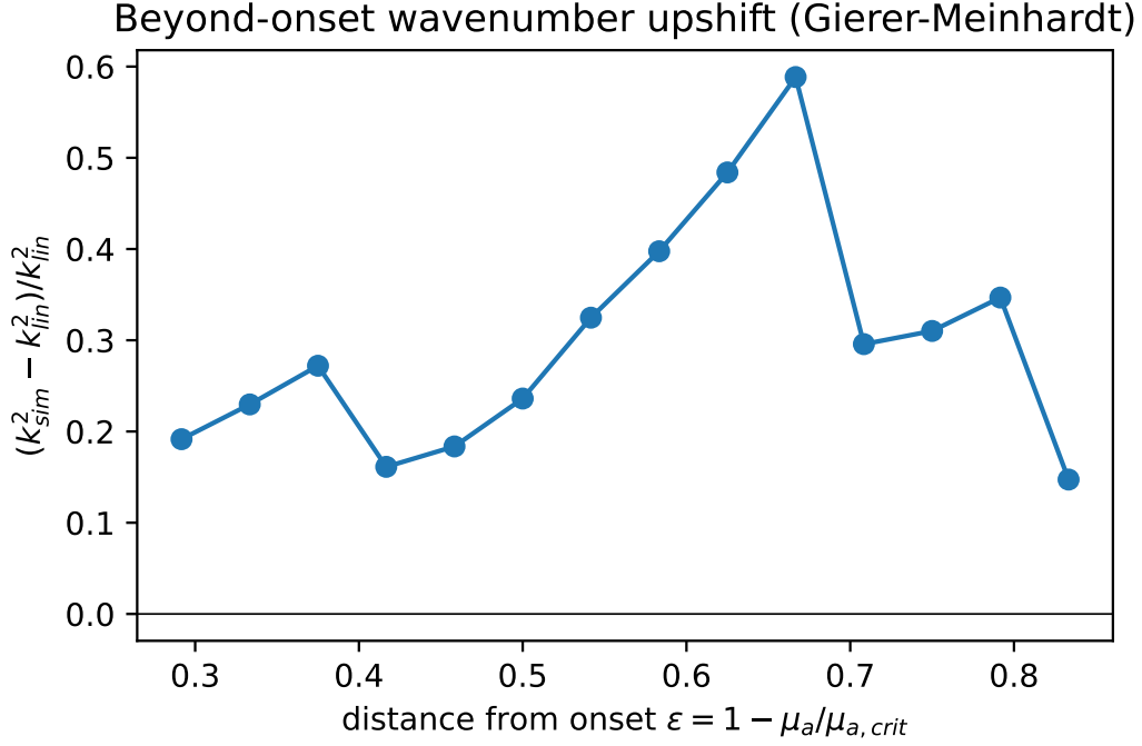
Figure 2: Selected vs. linear wavenumber across the sweep. Left: k_{sim}^2 against k_{lin}^2 (identity line shown). Right: relative deviation as a function of distance from onset \varepsilon ; the peak at intermediate \varepsilon is the phenomenon the CNN surrogate (below) failed to predict from linear information alone.
