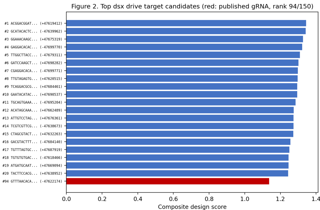
Figure 2. Top-20 v1 candidate sites (blue) and the published Kyrou gRNA at its true rank (red).
