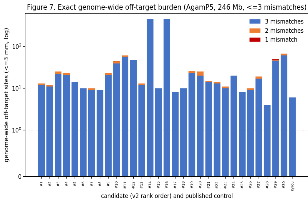
Figure 7. Exact genome-wide off-target burden of the v2 top-30 candidates and the published Kyrrou guide, stacked by mismatch class (symlog scale; AgamP5, 246 Mb, \leq 3 mismatches).
