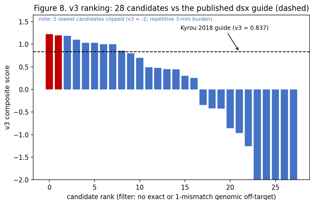
Figure 8. v3 composite ranking of the 28 filter-passing candidates against the published Kyrrou 2018 guide (dashed line, v3 = 0.837 ). Red: named lead candidates dsx-v3-1 and dsx-v3-2.
