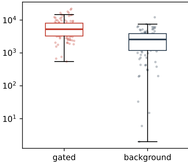
(b) systematic: expression MW p=2.5e-12
