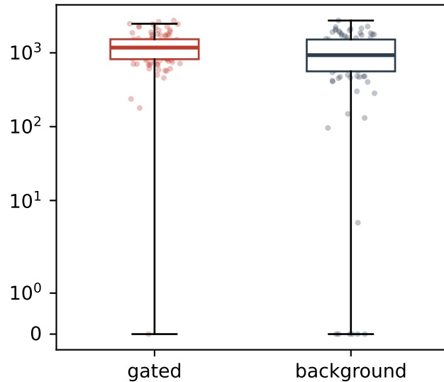
(c) systematic: non-expression MW p=0.017
