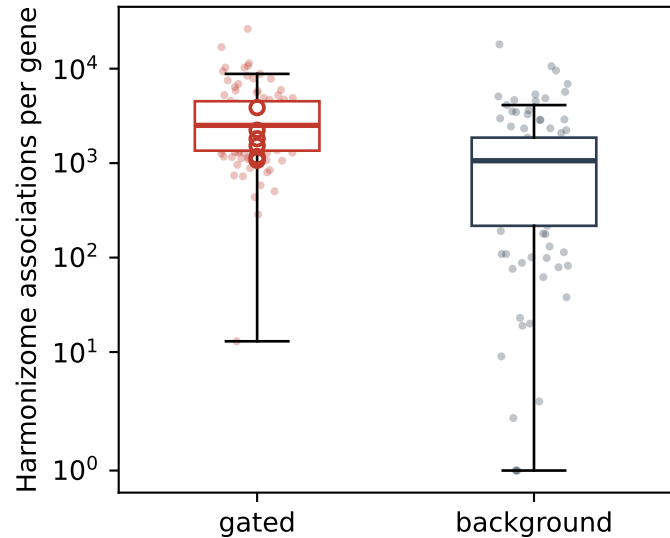
(a) curated/literature MW p=6.3e-10
