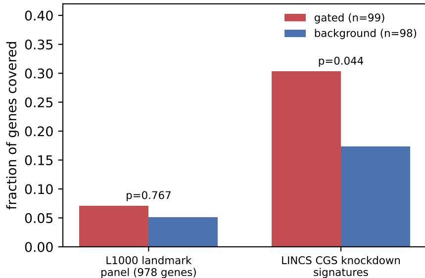
LINCS L1000 visibility of the gated surfaceome (AND-gate antigens: 0/7 landmark, 2/7 CGS)
