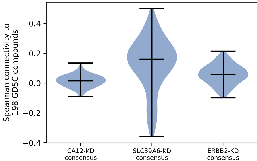
Connectivity-map pilot: positive control NOT recover (EGFR/HER2 inhibitors 1/20 top ERBB2 mimics, p=1 )
