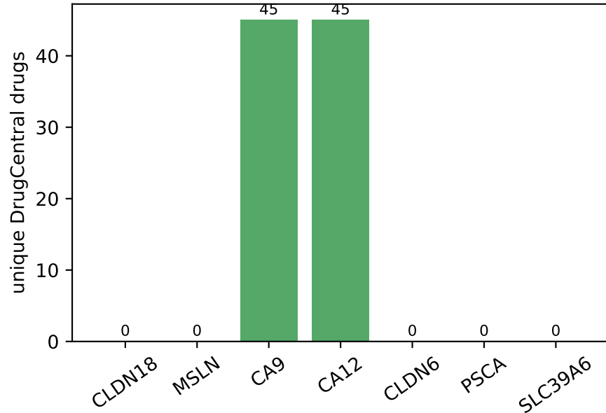
Gated vs random surfaceome: DrugCentral engagement (null) AND-gate antigens: quantitative engagement
