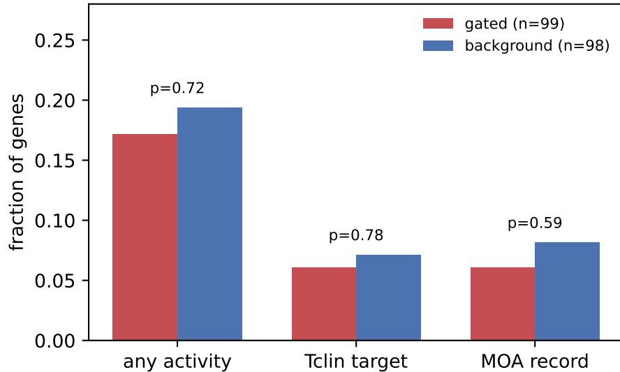
Gated vs random surfaceome: DrugCentral engagement (null) AND-gate antigens: quantitative engagement
