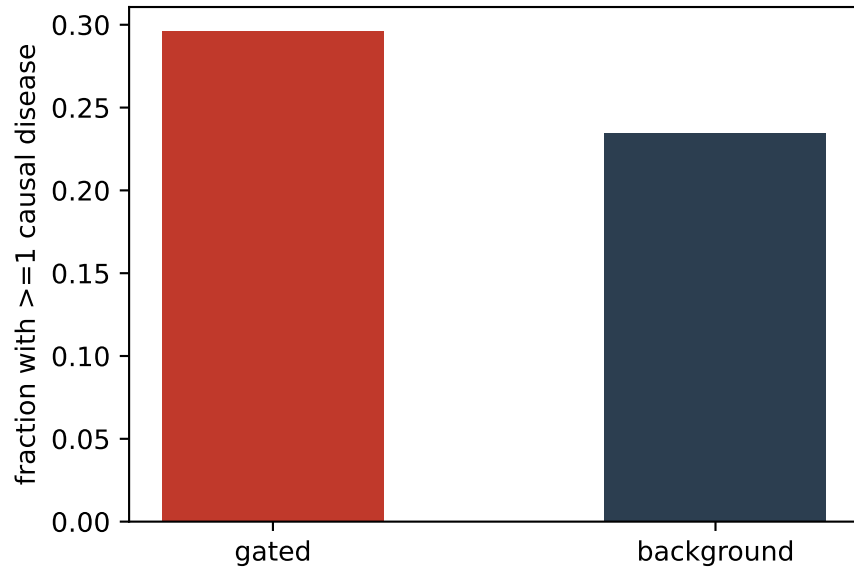
(a) Mendelian causal-disease carriers (Fisher p=0.419 )
