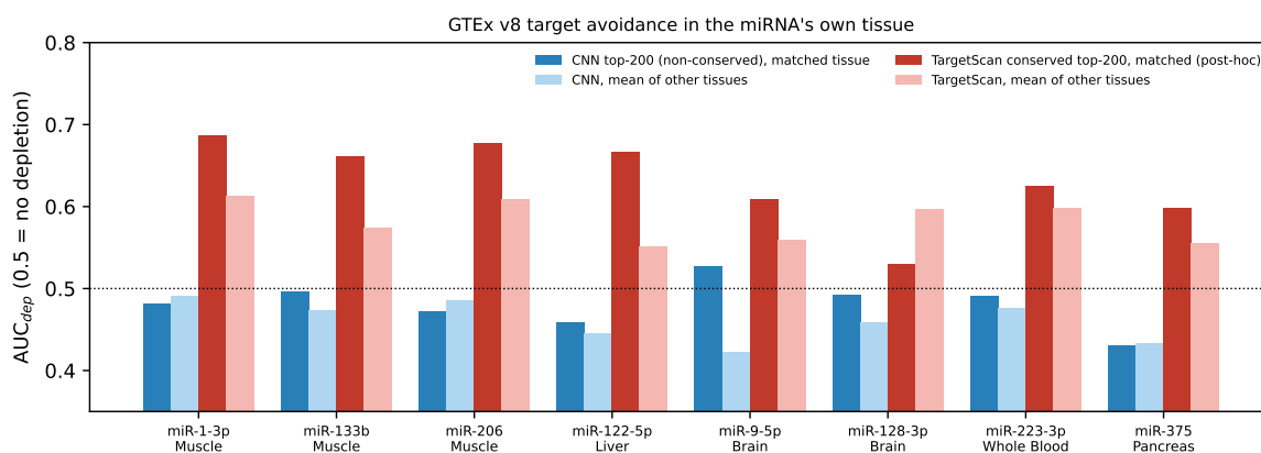
Figure 13: Depletion ( AUC_{dep} ) of target sets in each miRNA's own GTEx tissue versus the mean over the other design tissues. Blue: CNN top-200 in the CLIP universe (pre-registered). Red: TargetScan conserved top-200 in the all-UTR universe (post-hoc reference).
