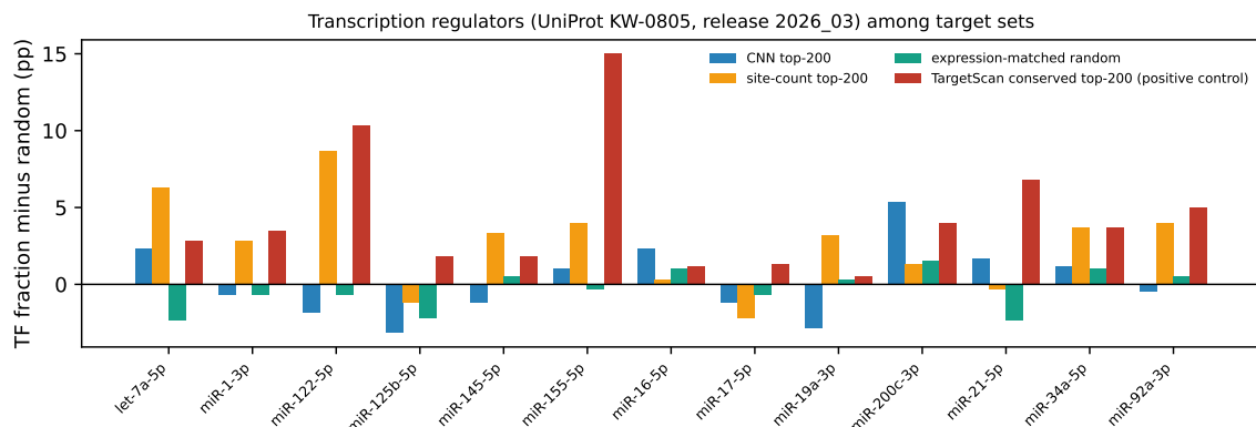
Figure 17: Transcription-regulator fraction of each 200-gene set minus its random baseline (percentage points). Red: TargetScan conserved targets against random UTR genes (positive control).
