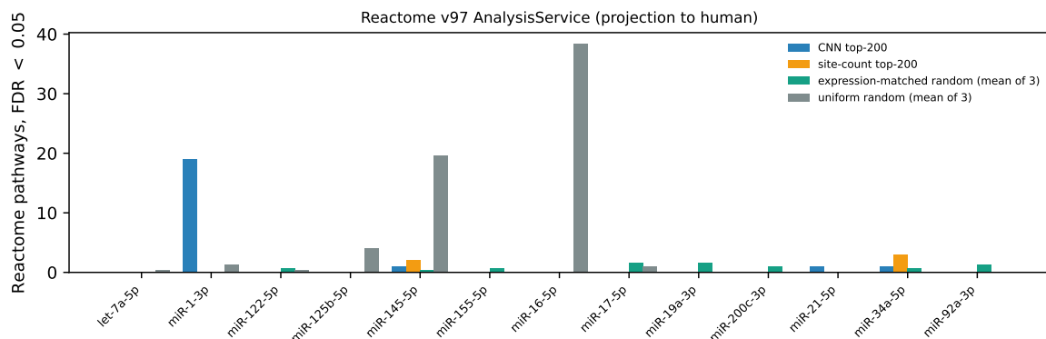
Figure 15: Significant Reactome pathways per miRNA for four arms of 200 genes. Gates G1 and G3 failed, so these counts are descriptive.
