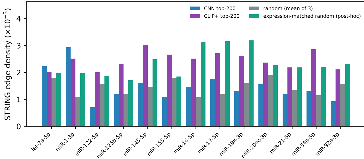
Target-set network density (STRING v12, score \geq 0.7 )
