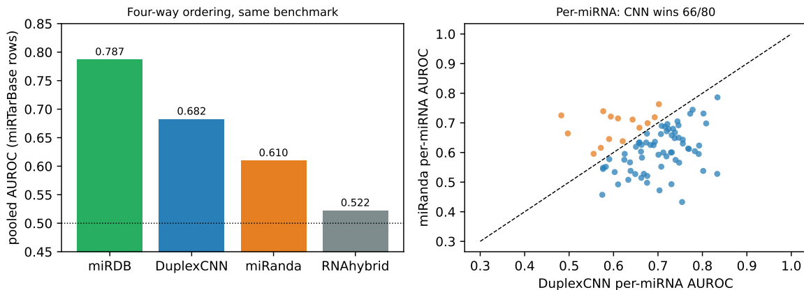
Figure 9: Left: pooled AUROC on the committed miRTarBase rows for the four predictor arms (miRDB from results/mirdb.benchmark.json; the other three on identical rows, n = 7,914 ). Right: miRanda versus DuplexCNN per miRNA; orange points are miRNAs where miRanda wins.
