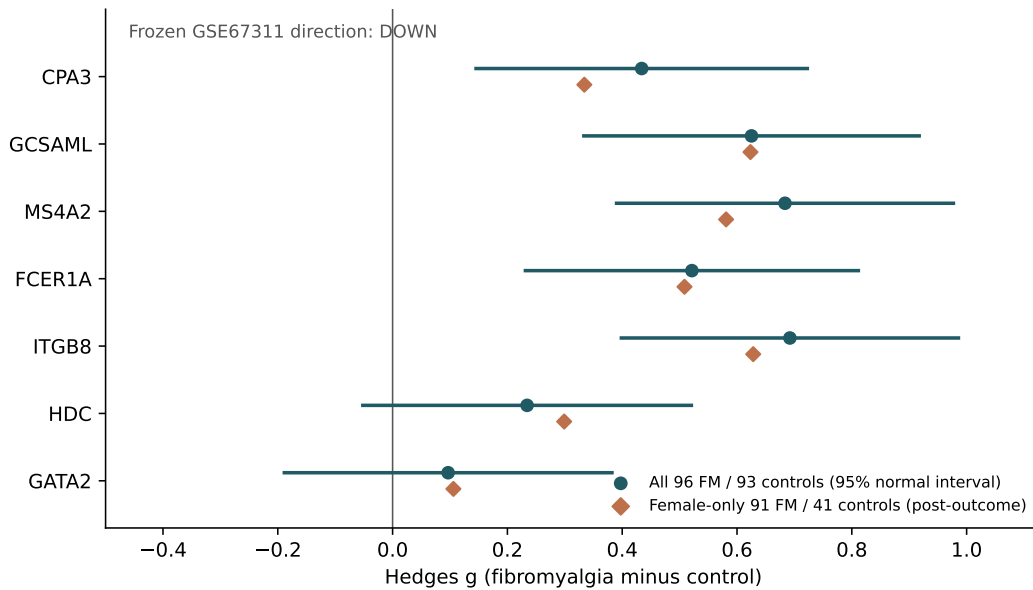
Figure 5: Frozen GSE67311 fibromyalgia DOWN candidates in GSE221921. All seven uniquely measured genes reverse UP. Teal dots and normal-reference intervals are full-cohort Hedges effects; orange diamonds are female-only estimates added after the full-cohort result. The female sensitivity is descriptive, not a new validation cohort or evidence for opposite-direction clinical markers. UQCC3 is absent from the uniquely mapped source.
