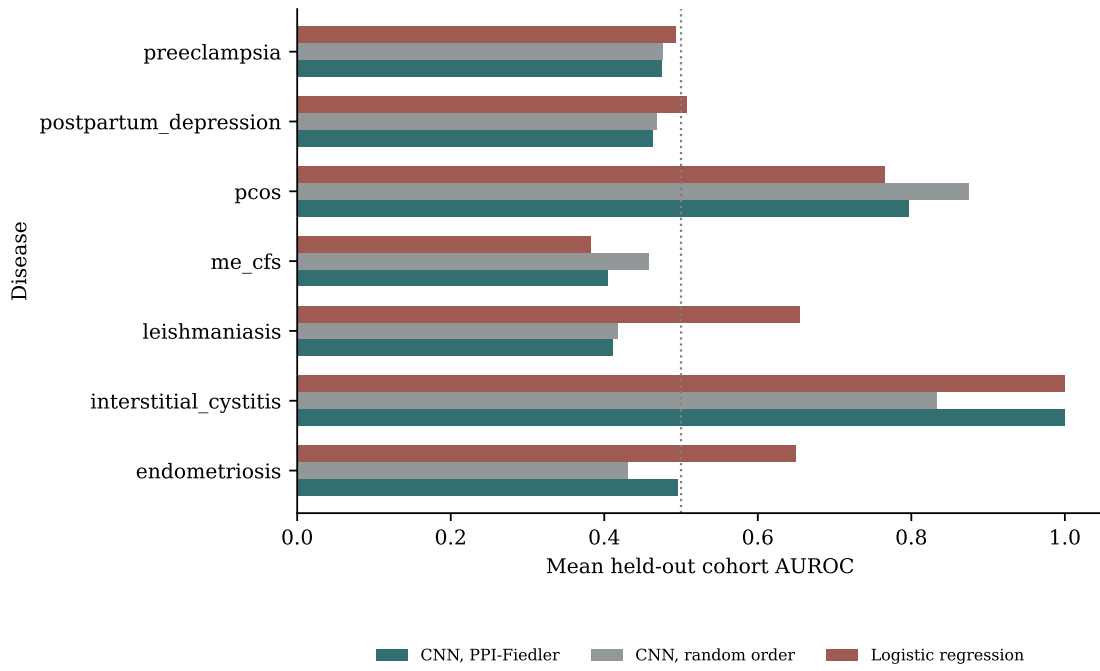
Figure 1: Held-out cohorts by disease, calculated from results/cnn_crosscohort.csv after deduplication. Historical pre-seeding result; corrected CNN scores appear in the later seeded-rerun section. Mean AUROC is unweighted across validation cohorts within each disease; cohort sizes differ.
