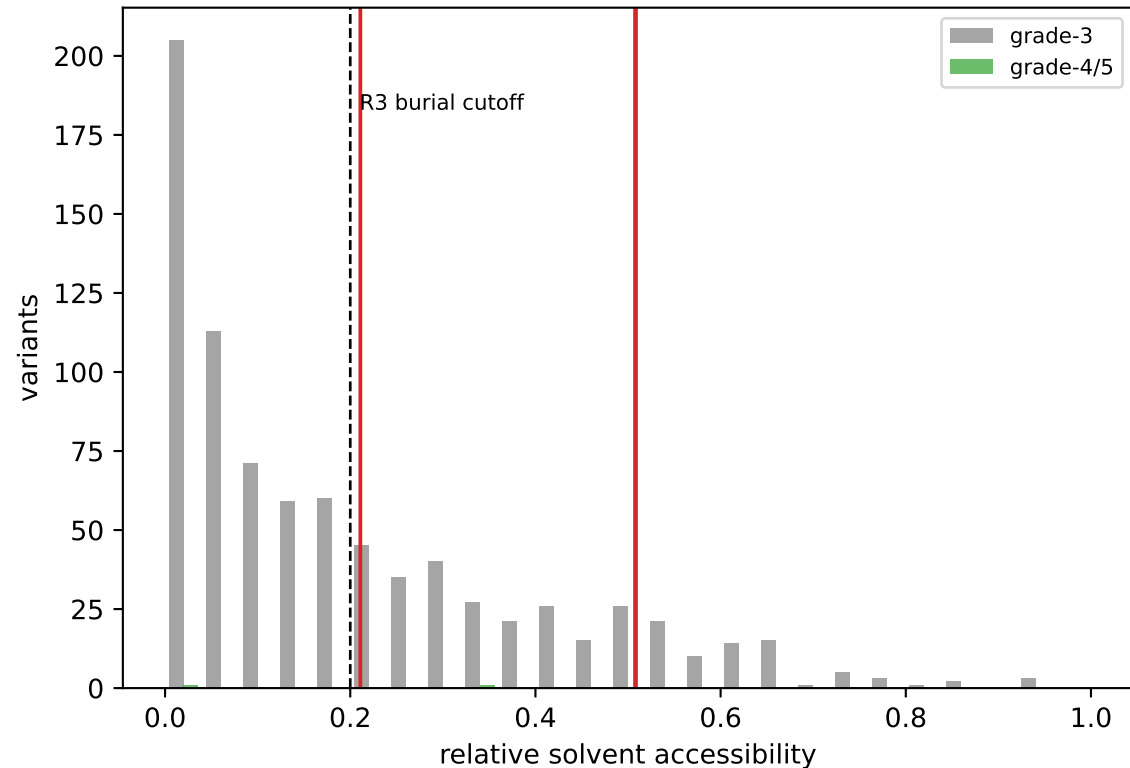
Burial by WHO grade
