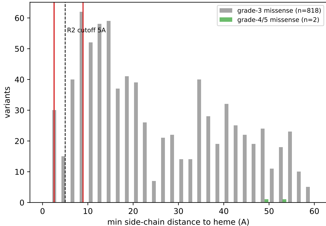
Heme proximity by WHO grade (red = 5 grade-1/2 missense)
