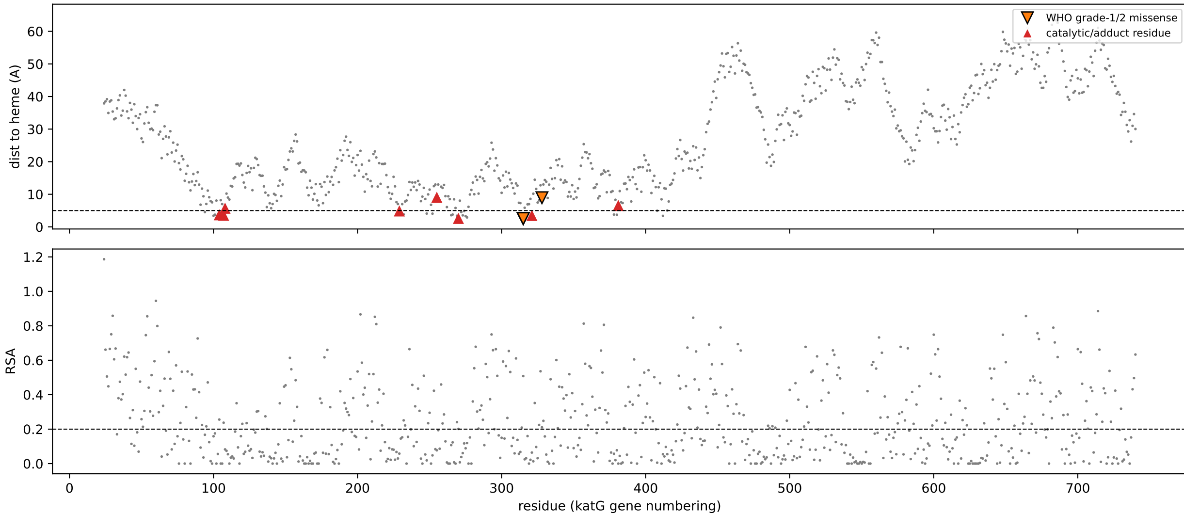
katG per-residue structural profile (1SJ2 chain A)
